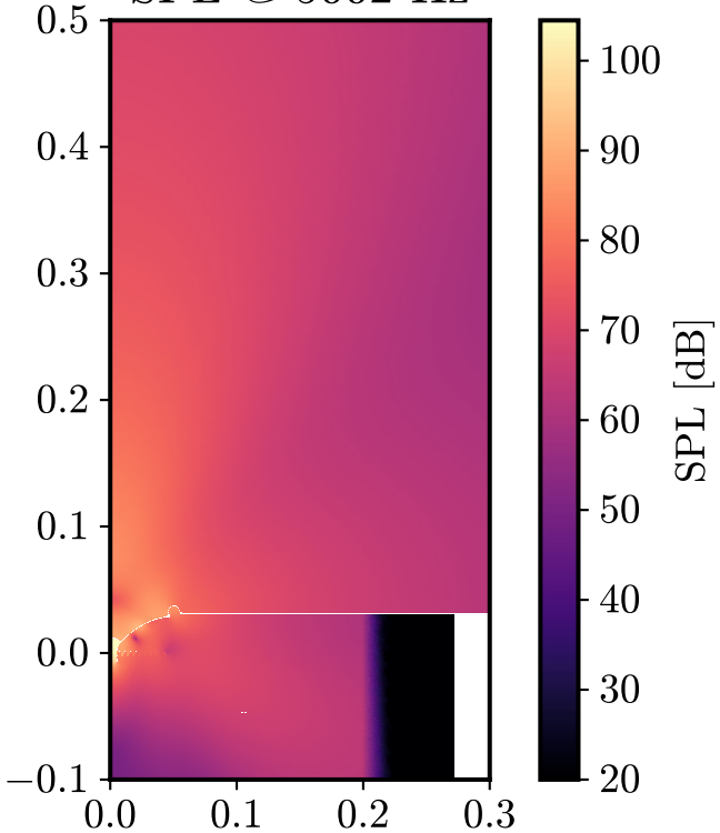
SPL @ 5002 Hz
