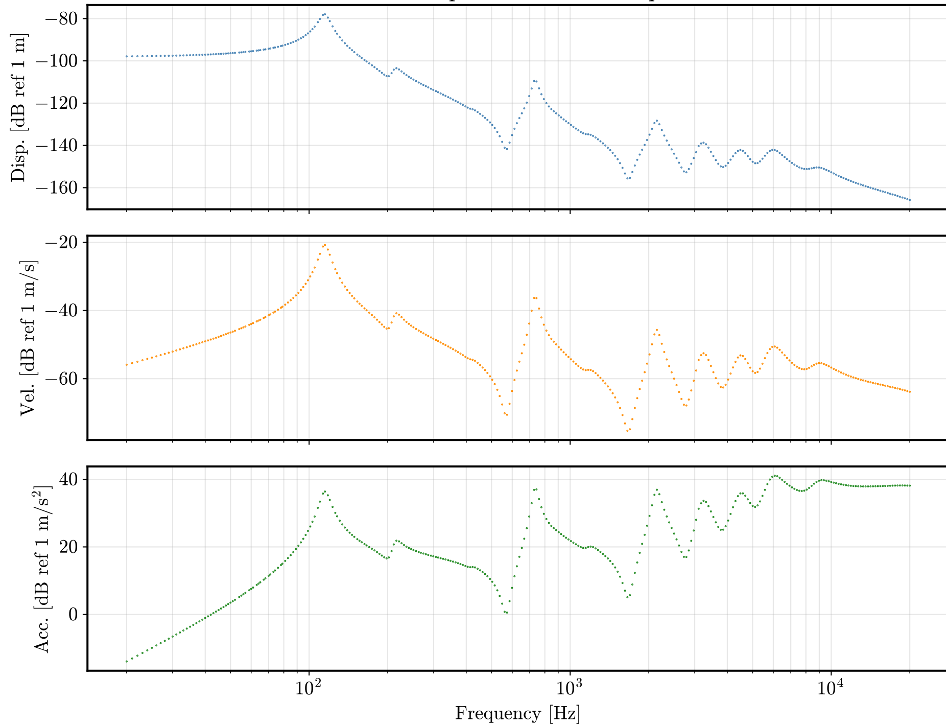
Cone tip - mechanical sweep
