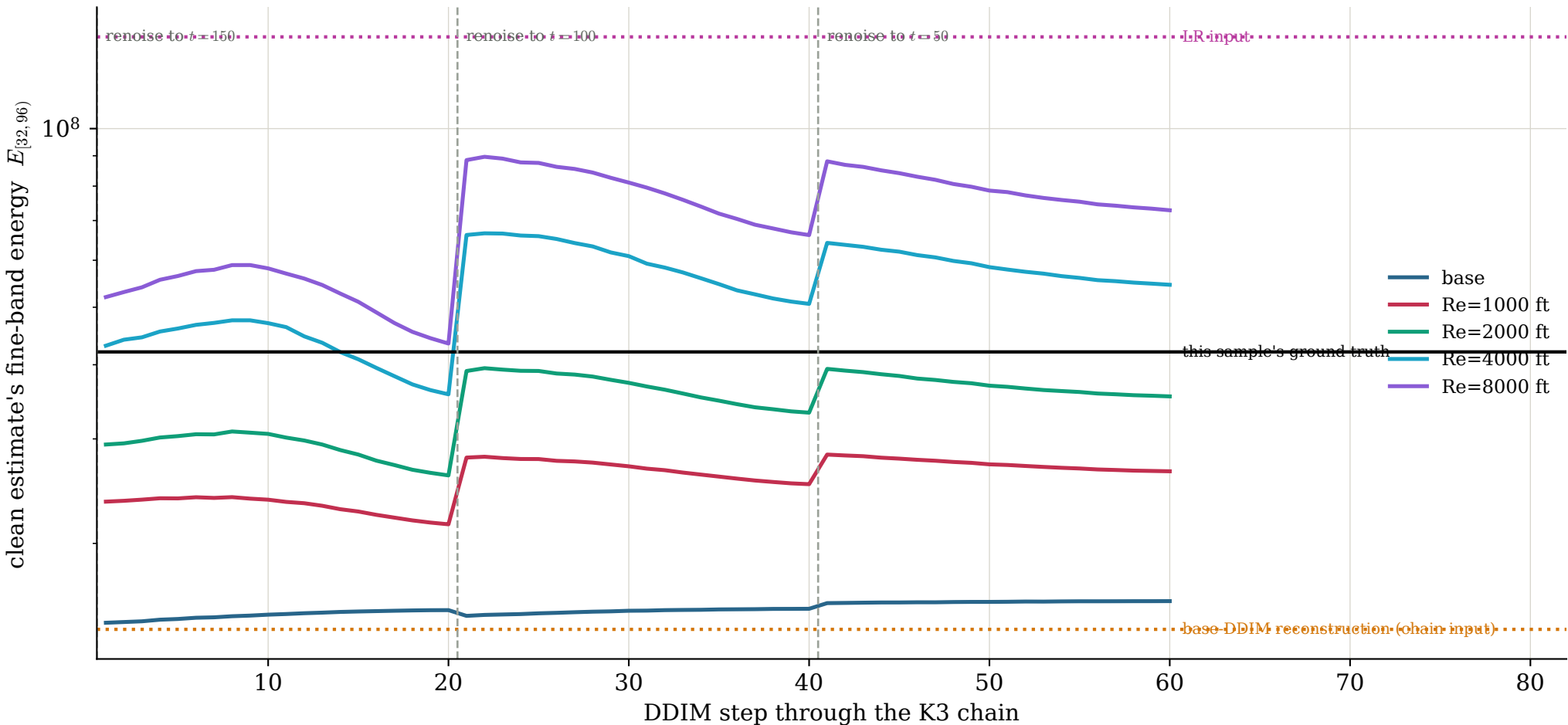
One sample (test triplet 27) through the full K3 chain, every model, identical noise the energy level is set at each re-noising pass and holds within it
