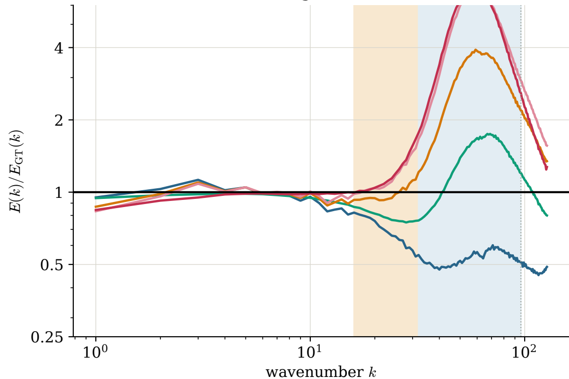
The Re=8000 specialist at Re=1000, unguided: each chain rung is a dose mean vorticity spectrum
