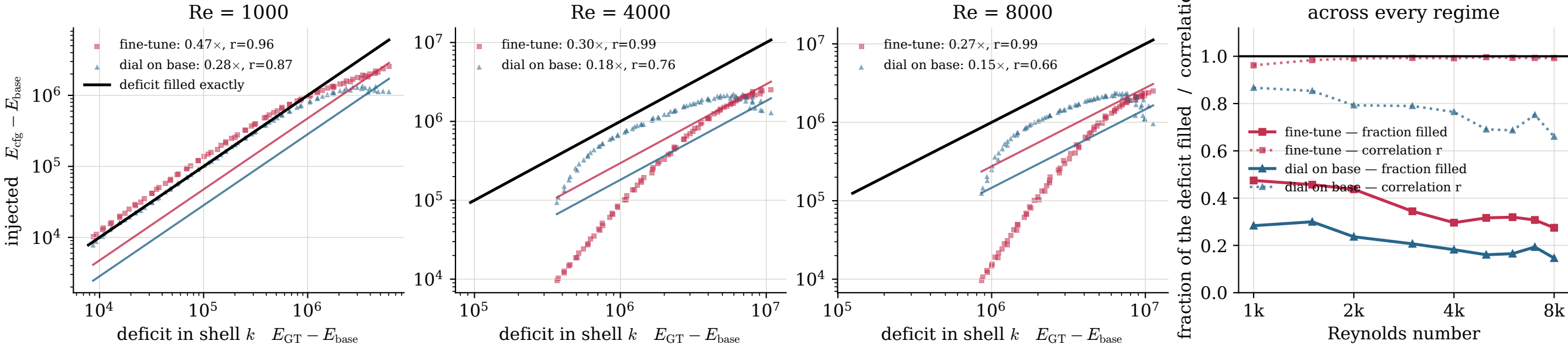
Does the injected energy go where it is missing? Shells k \in [16, 96) , one point per shell
