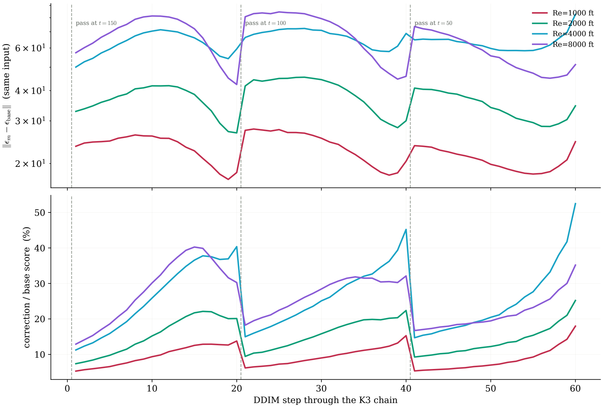
The magnitude of the fine-tuned correction through the chain (test triplet 27, real sampler)
