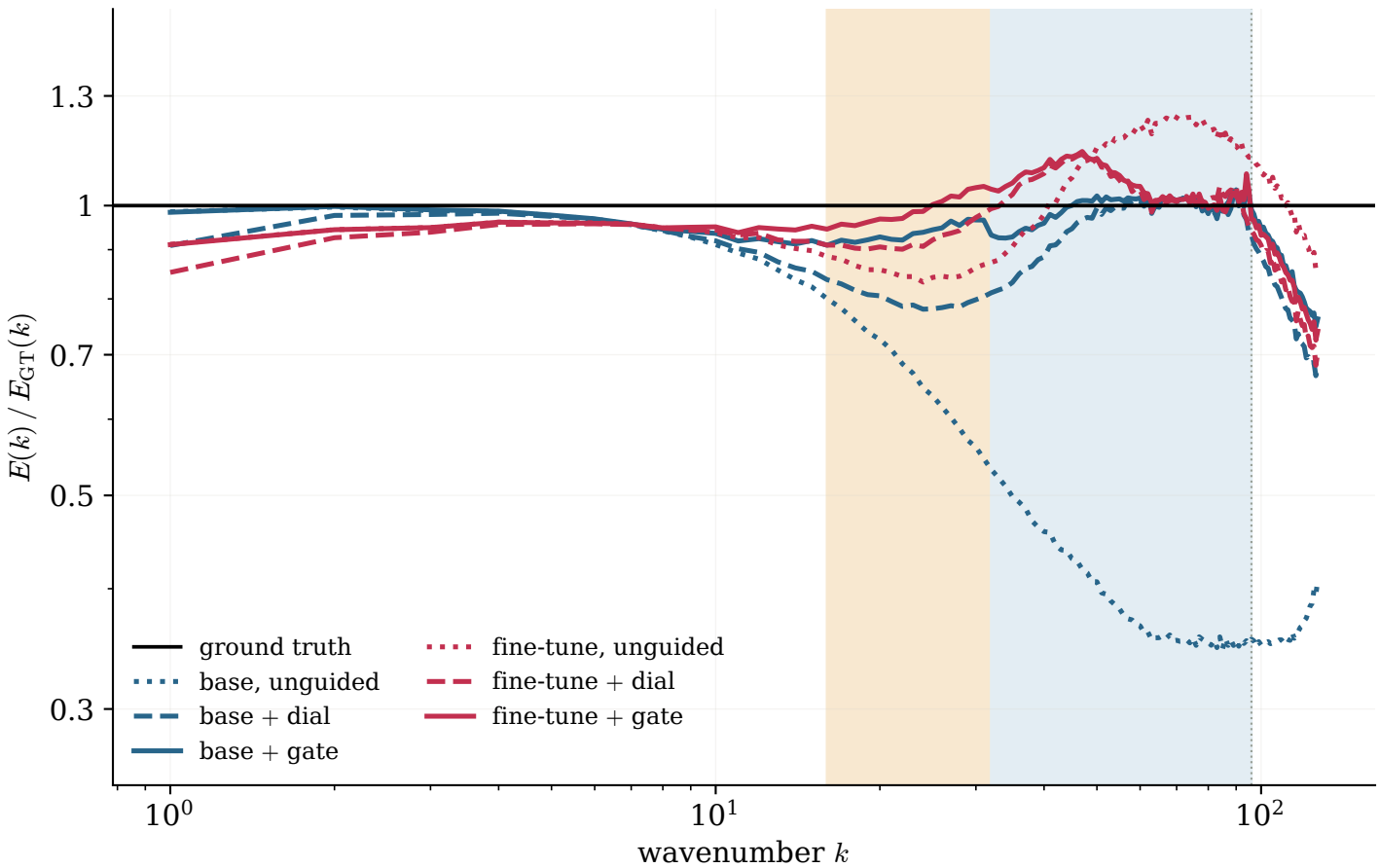
Tapered dial against the per-band per-sample gate, Re=1000
