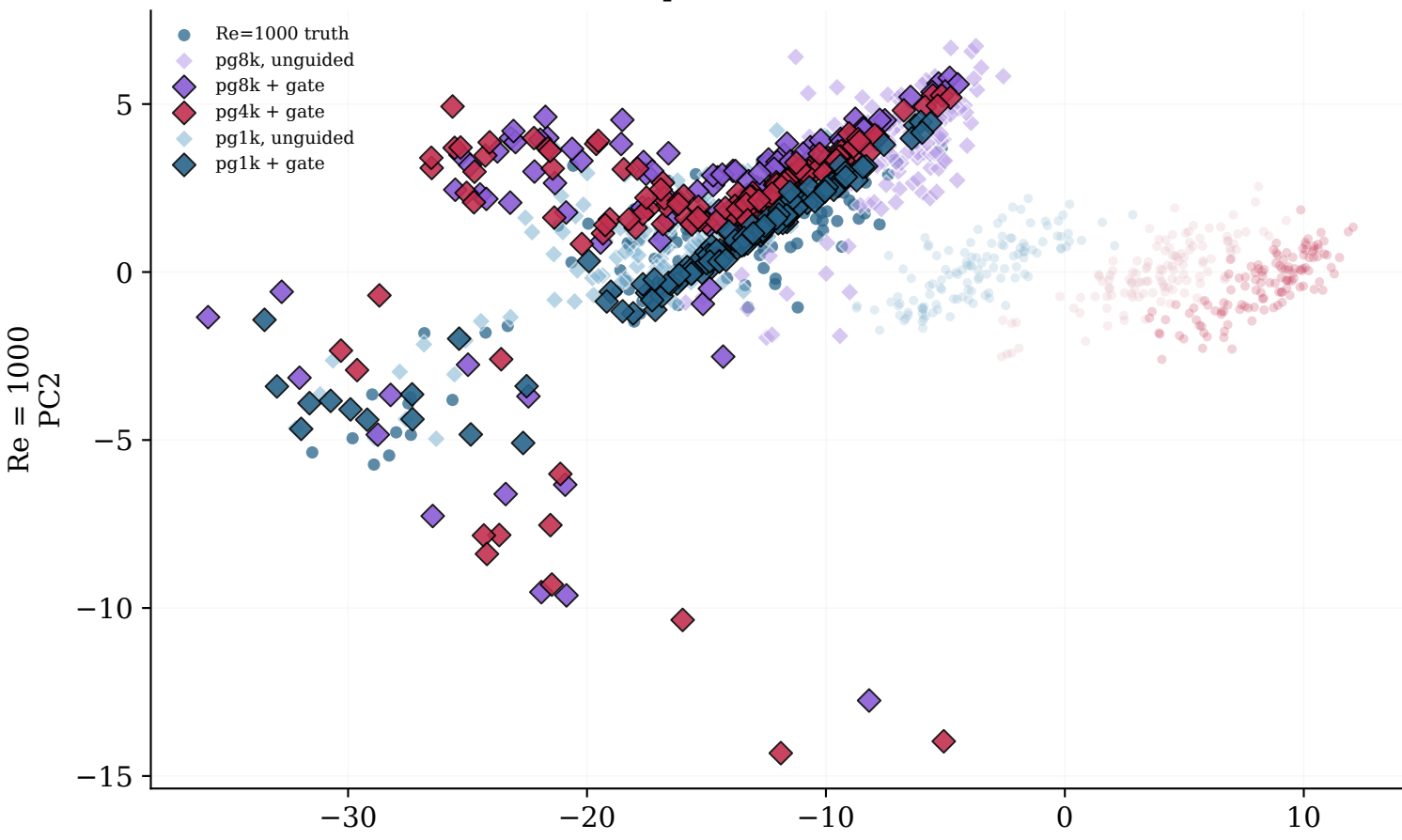
Pure-gate specialists across the ladder, manifold clouds and spectra
