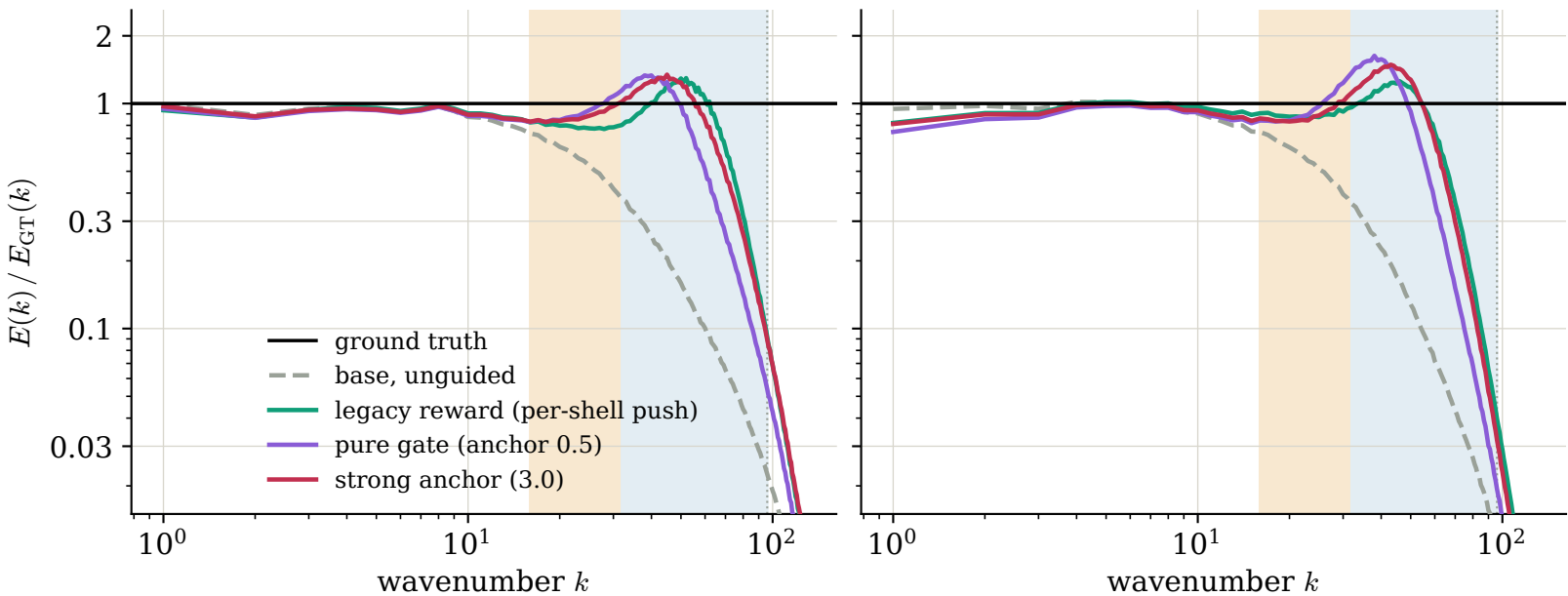
Ratio to ground truth, Re=4000, Re=8000
