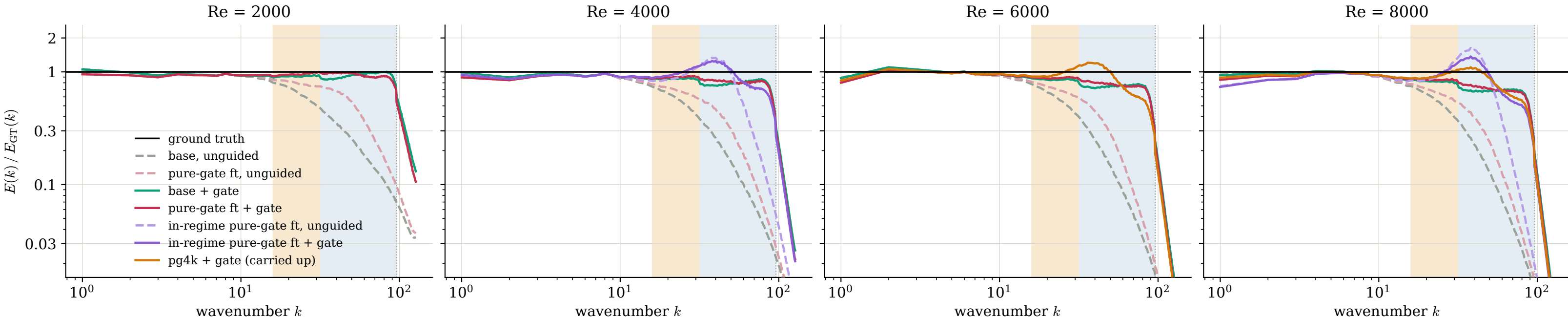
Ratio to ground truth, Re=2000, Re=4000, Re=6000, Re=8000
