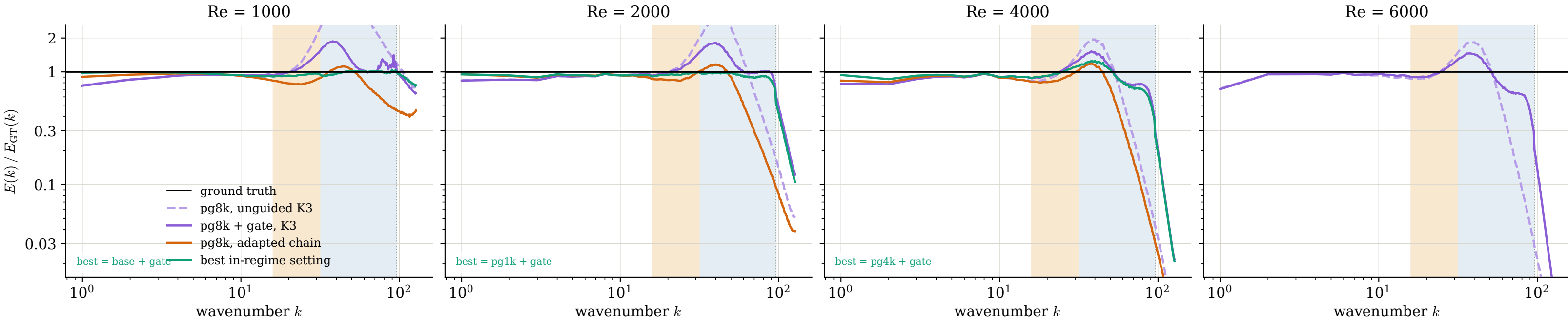
Ratio to ground truth, Re=1000, Re=2000, Re=4000, Re=6000
