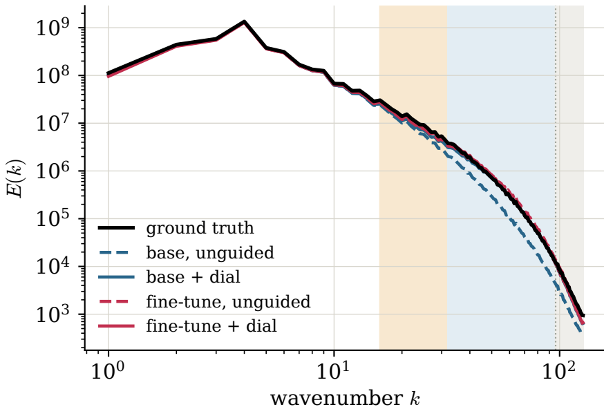
In distribution (Re=1000), unguided and with the tapered dial mean vorticity spectrum
