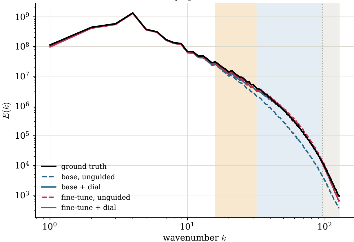
Mean vorticity spectrum, Re=1000
