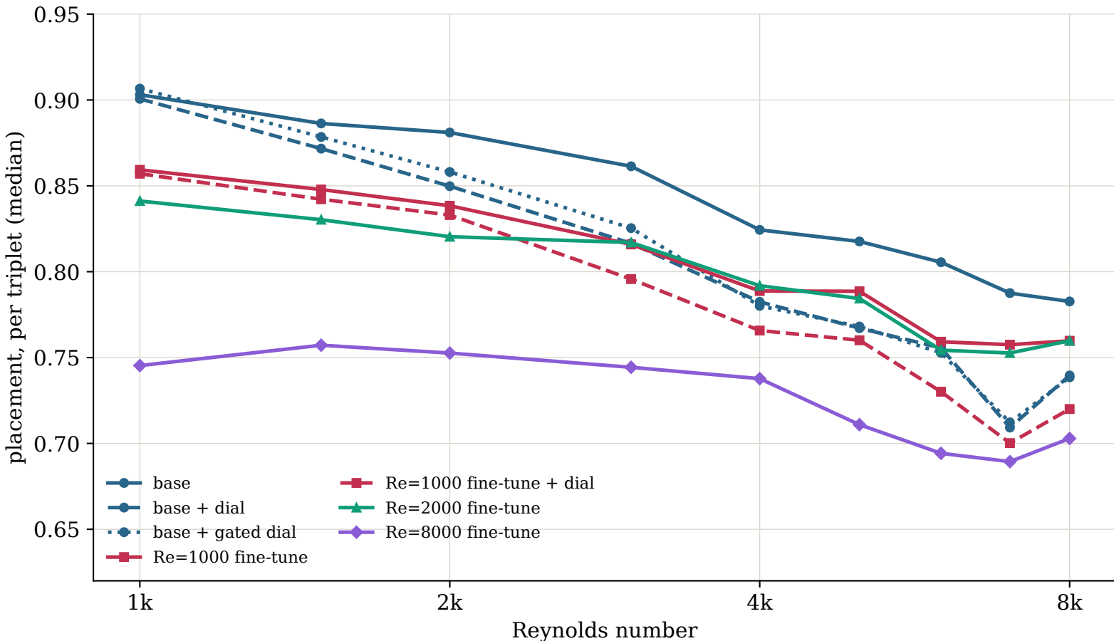
Spatial placement of the small scales ( k \geq 32 highpass, \sigma = 6 ), against Reynolds number
