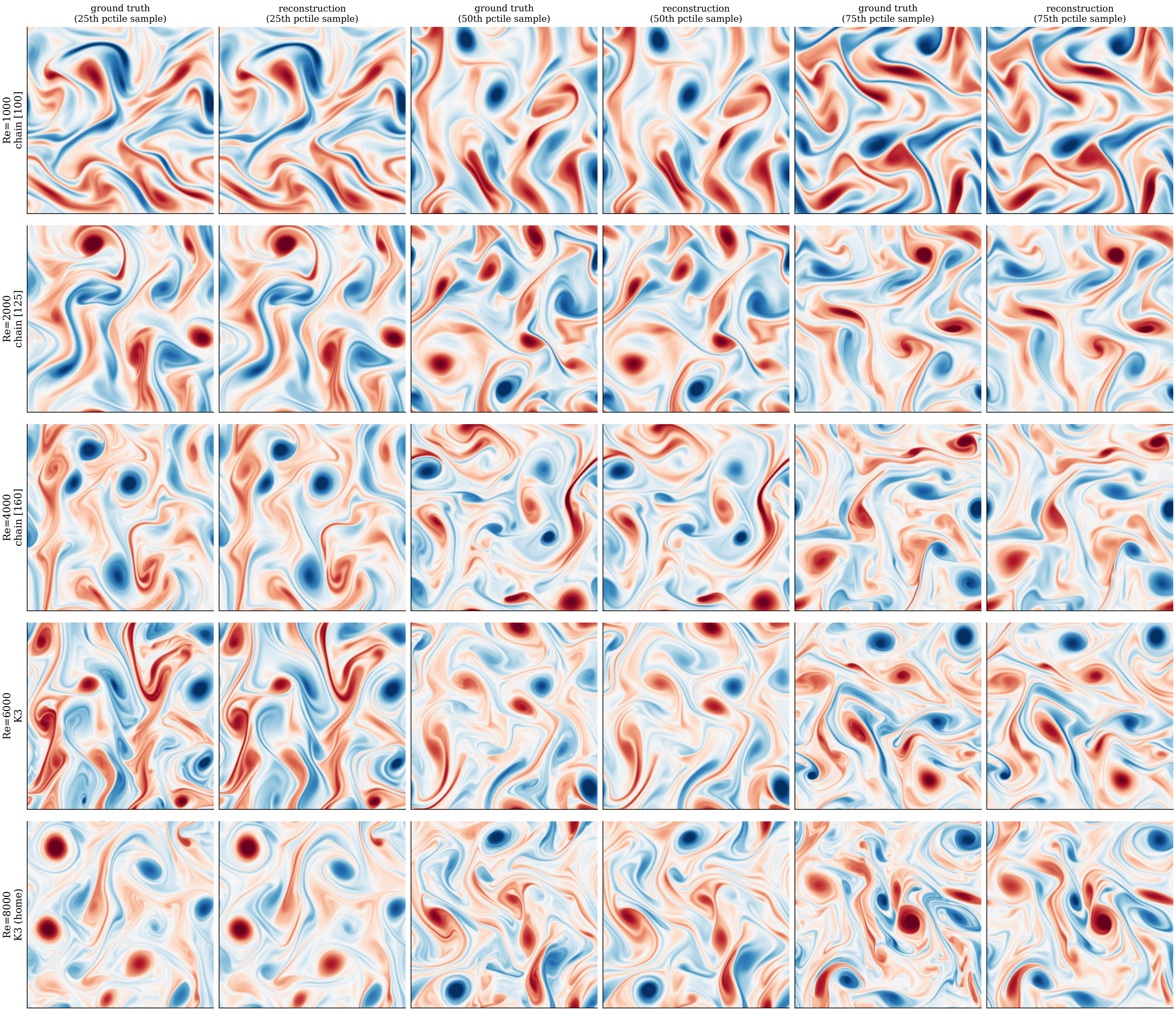
The Re=8000 fine tune across the ladder under the selected inference configuration per regime, three samples per regime (vorticity)
