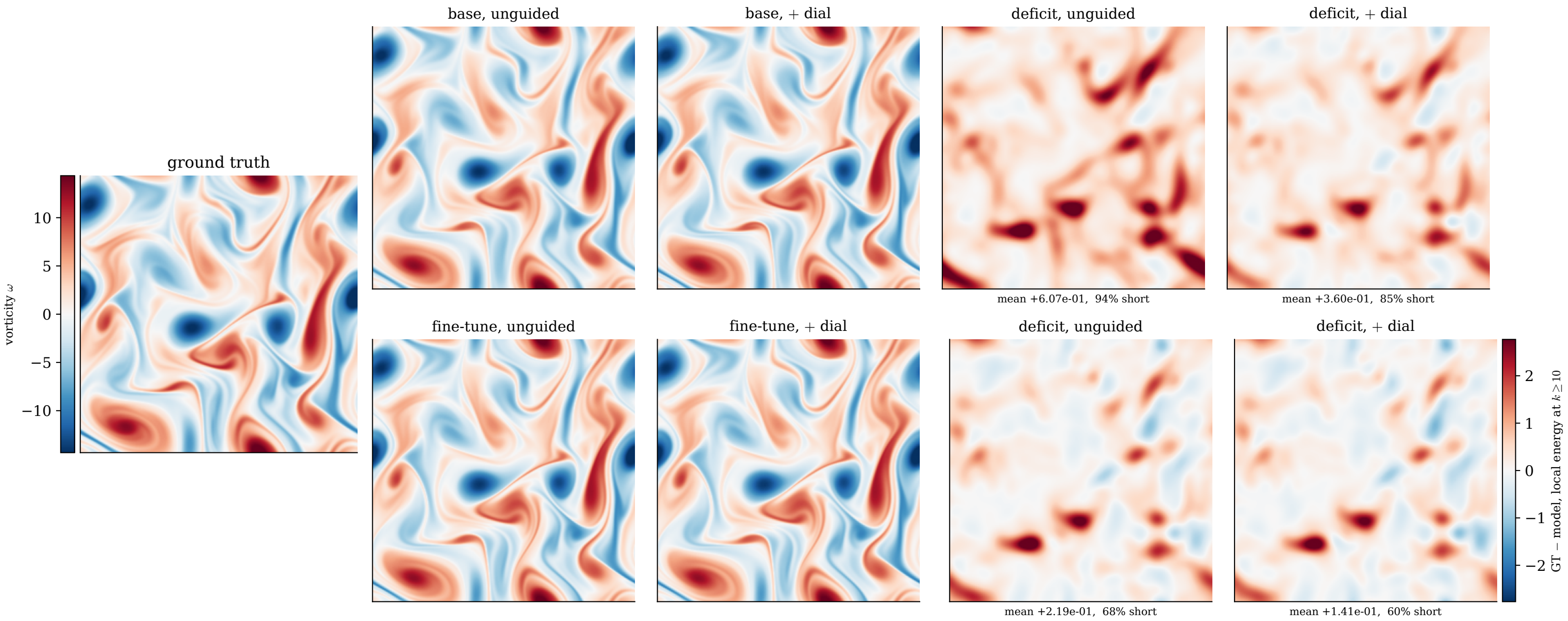
Reconstructions and fine-scale deficit with and without the tapered dial — Re=1000, held-out triplet 31 (red = missing, blue = excess)
