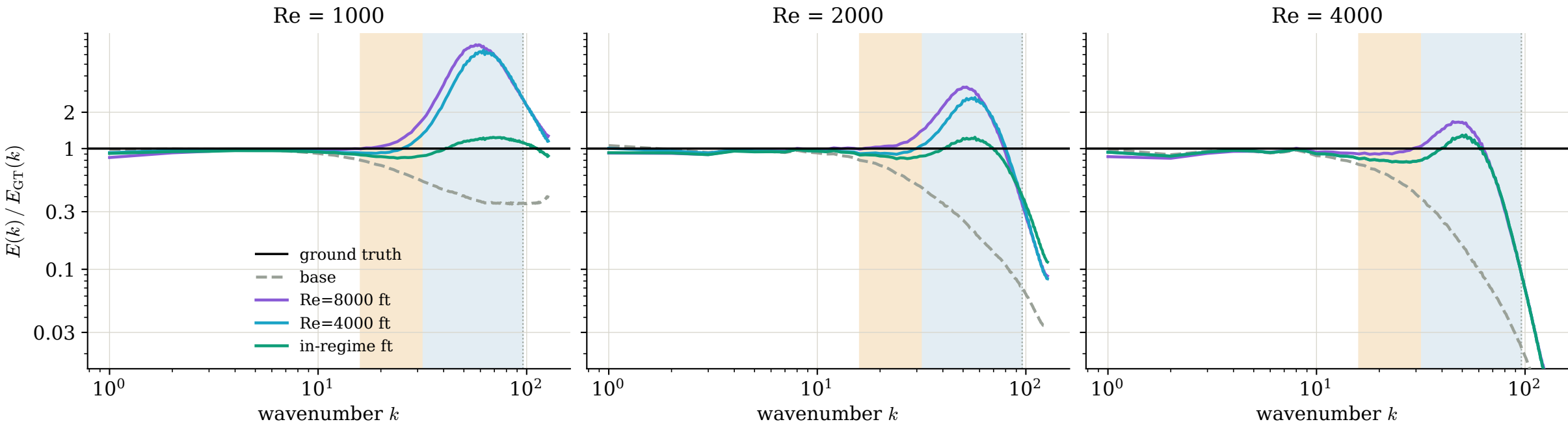
Ratio to ground truth, Re=1000, Re=2000, Re=4000
