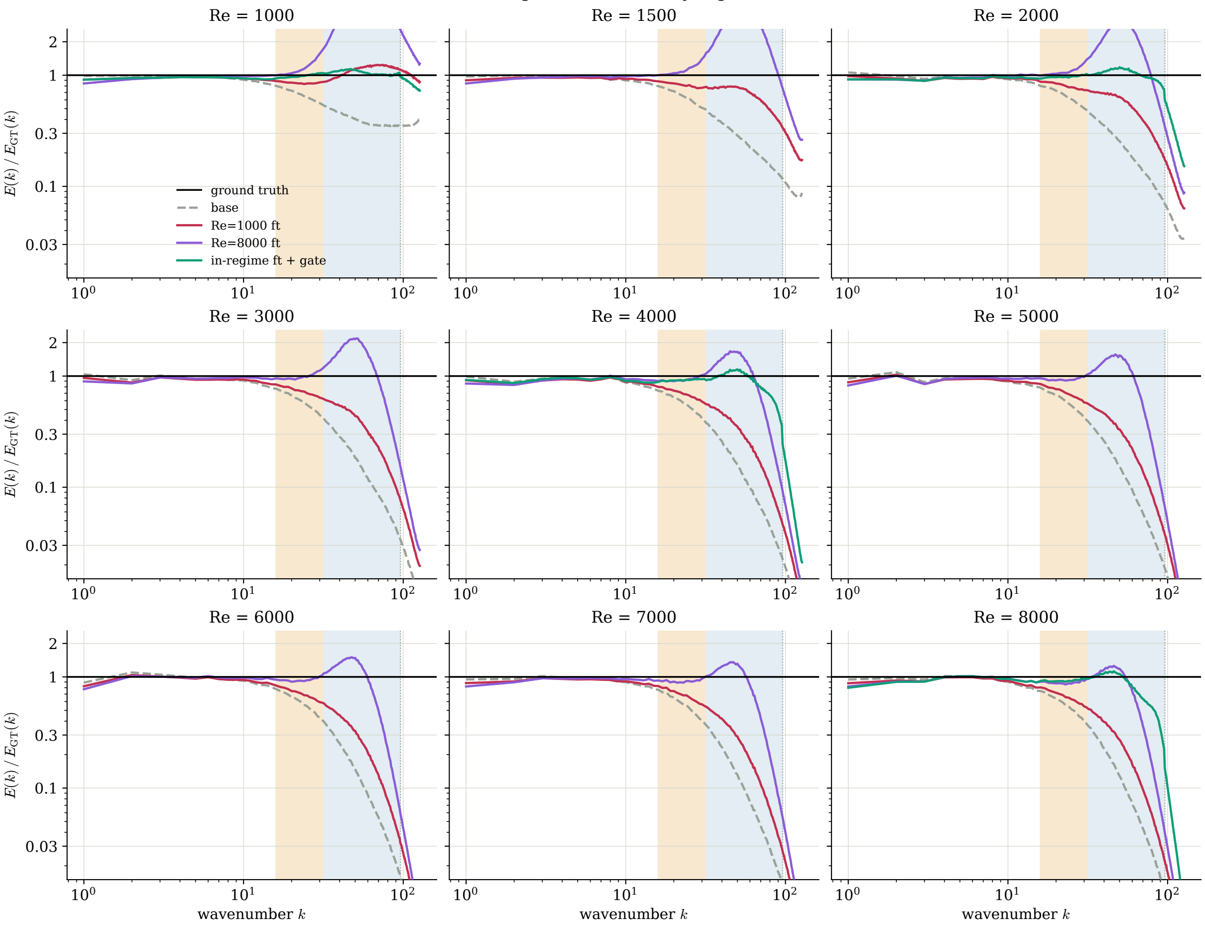
Ratio to ground truth, every regime
