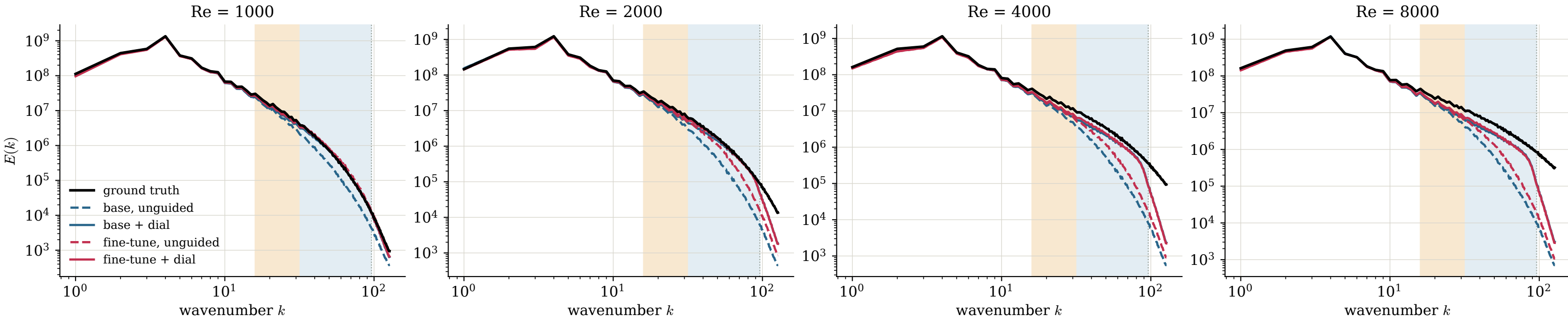
Mean vorticity spectrum, Re=1000, Re=2000, Re=4000, Re=8000
