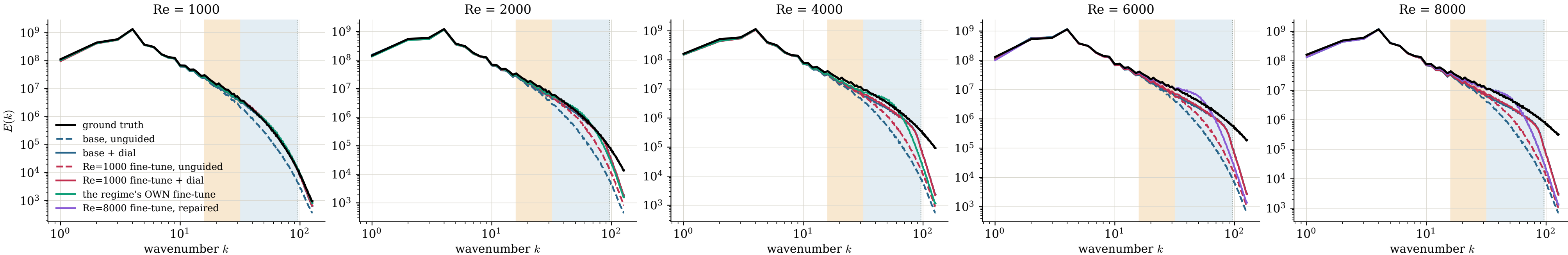
Mean vorticity spectrum, Re=1000, Re=2000, Re=4000, Re=6000, Re=8000
