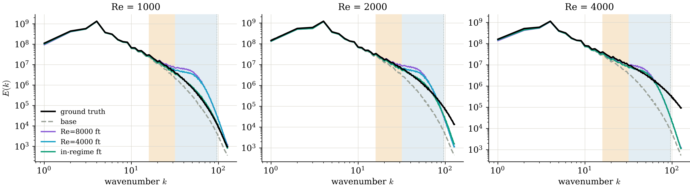
Mean vorticity spectrum, \text{Re}=1000 , \text{Re}=2000 , \text{Re}=4000
