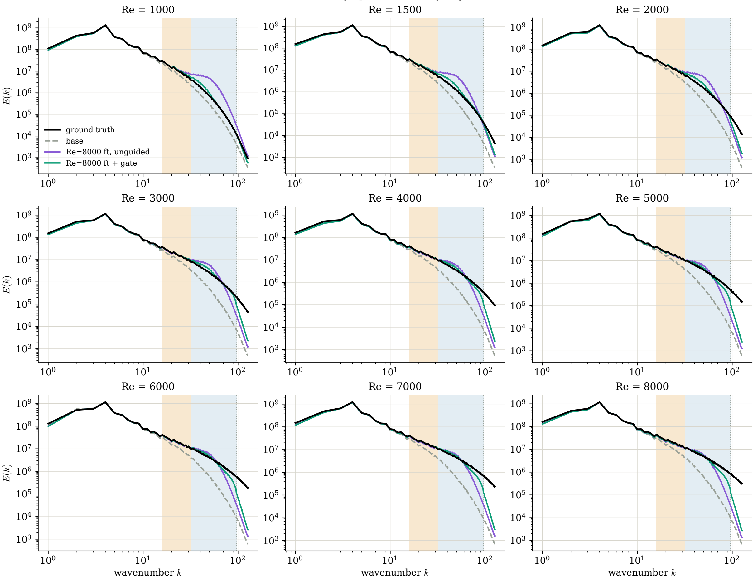
Mean vorticity spectrum, every regime
