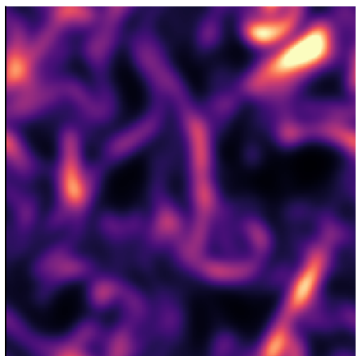
GT fine-scale energy ( k \geq 32 )
