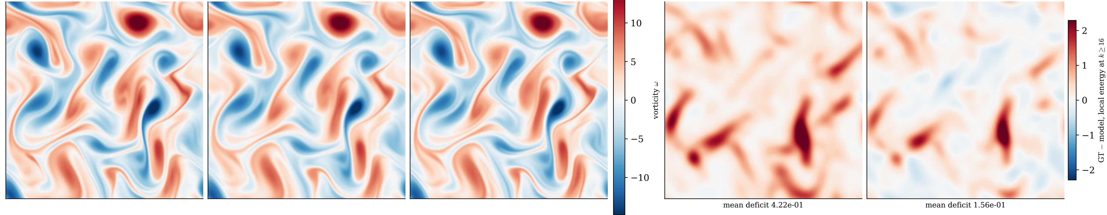
ground truth
