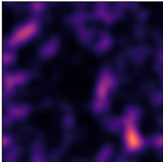
unguided
