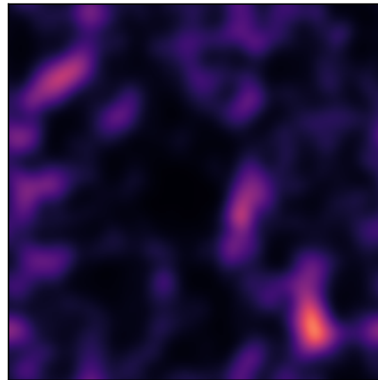
steered
