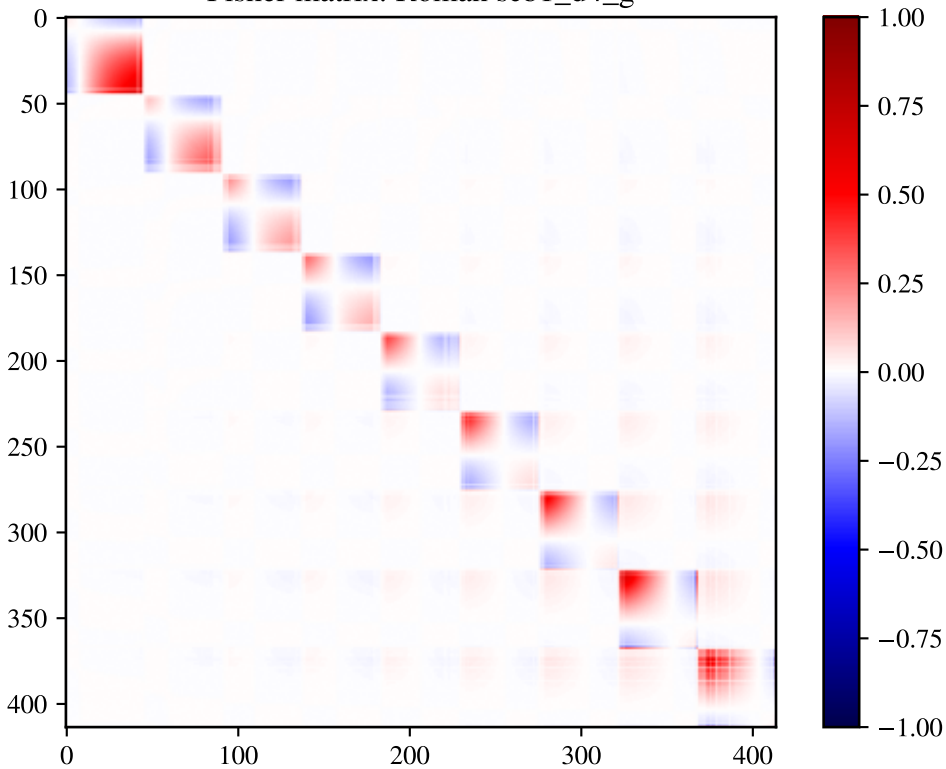
Fisher matrix: Roman scb1_d4_g
