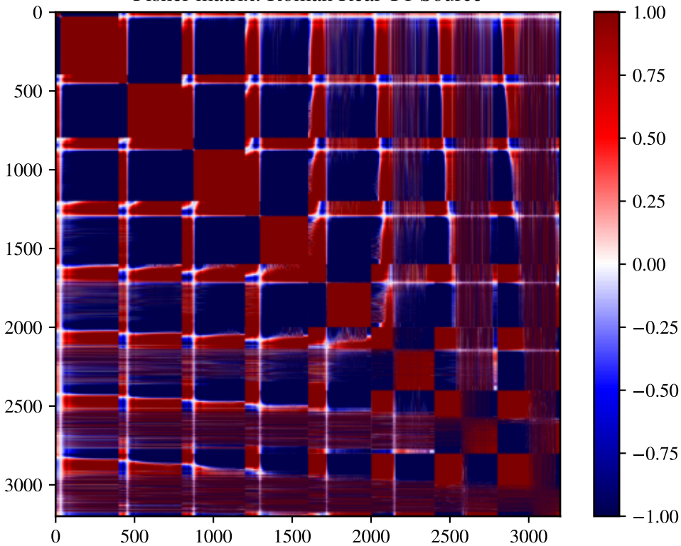
Fisher matrix: Roman Real Y1 Source
