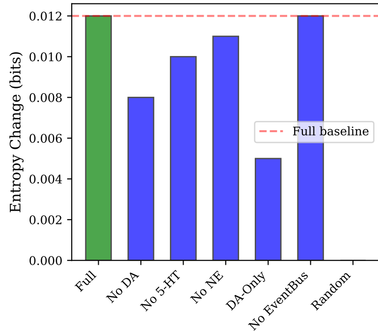
(a) Routing Entropy Under Stress
