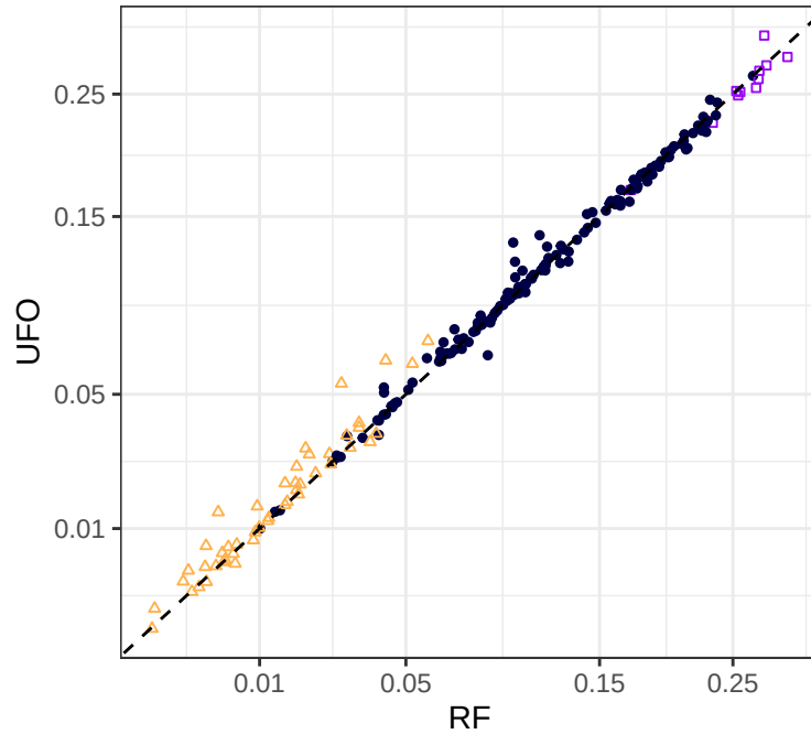
Brier
