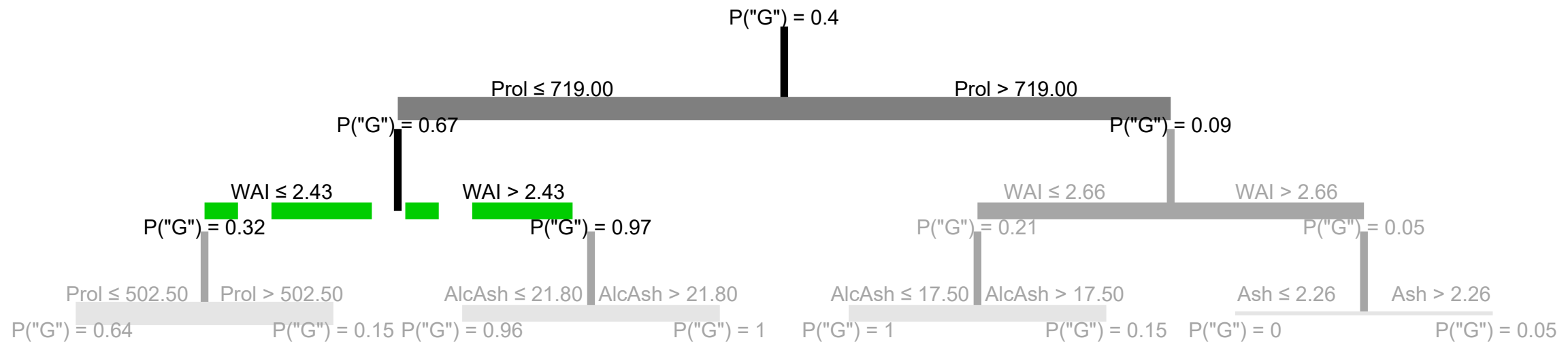
Influence of WAI for subgroup 'Prol \leq 719.00 '
