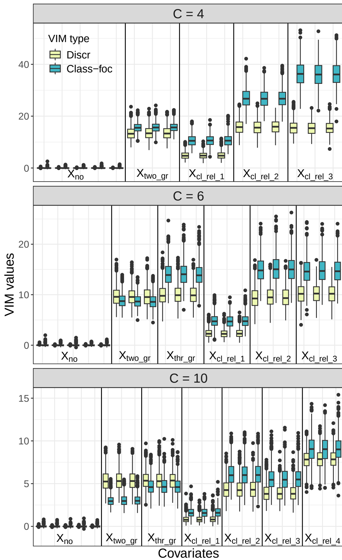
Class-focused and discriminatory VIM
