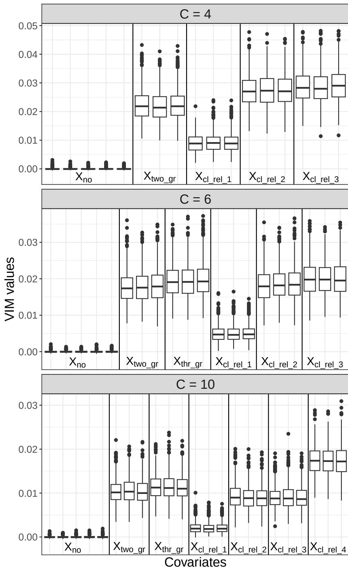
Permutation VIM
