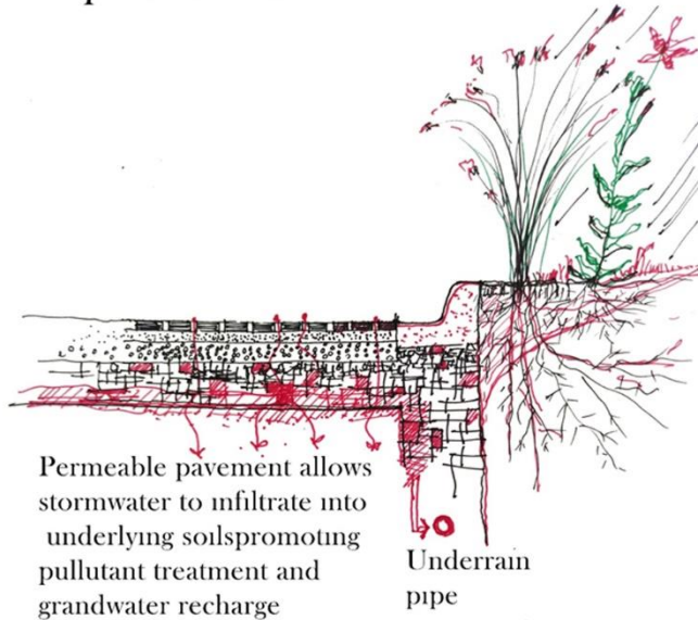
Permeable pavement diagram
