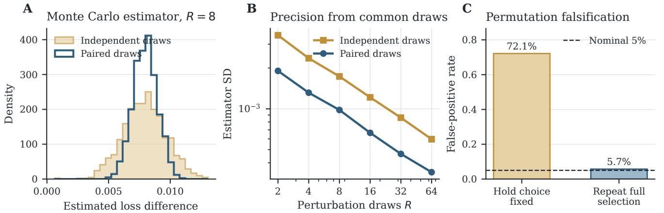
Figure 2: Pairing improves precision; full-workflow permutation restores nominal calibration in this controlled simulation. (A) Sampling distributions of the depth-three minus depth-four loss contrast at severity \lambda = 0.42 , using eight draws and a pool of 1,200 deterministic perturbations. (B) Estimator standard deviation over 900 Monte Carlo resamples at each R . (C) Null false-positive rates for a selected random predictor when model choice is held fixed versus repeated inside every permutation.
