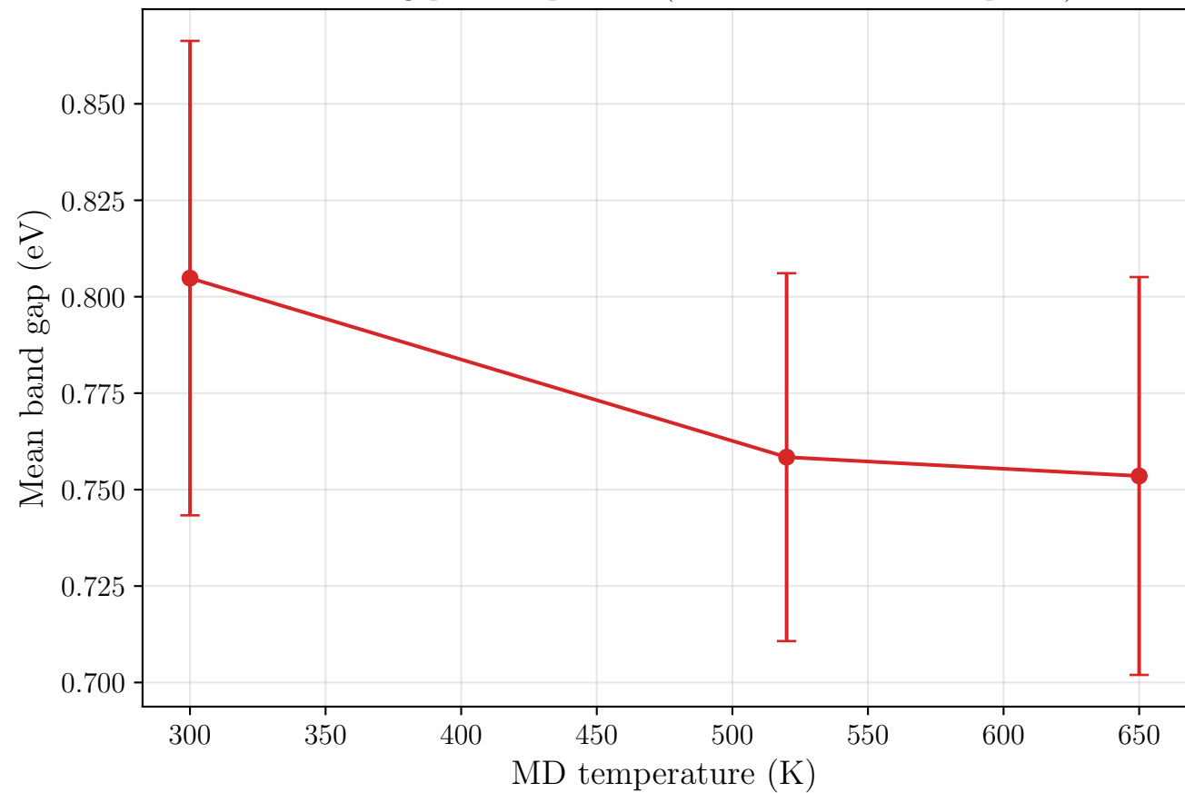
Mean band gap vs. temperature (error bars = std over snapshots)
