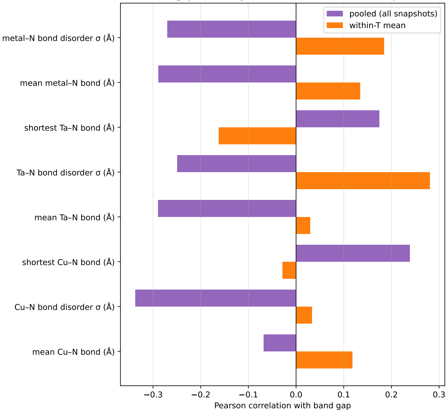
Band-gap sensitivity to interatomic-distance descriptors
