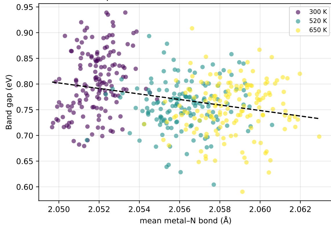
mean Cu-N bond ( \text{\AA} ) pooled r = -0.07 , within-T r = 0.12
