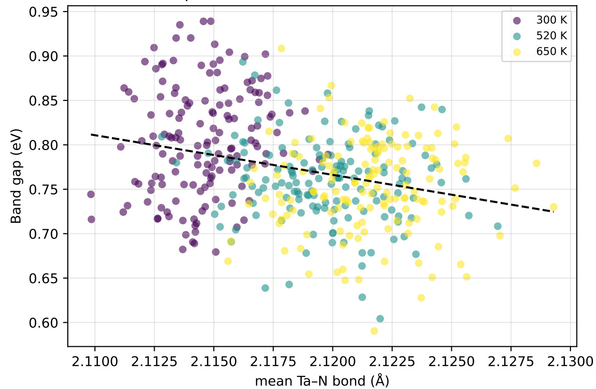
mean Ta-N bond ( \text{\AA} ) pooled r = -0.29 , within-T r = 0.03
