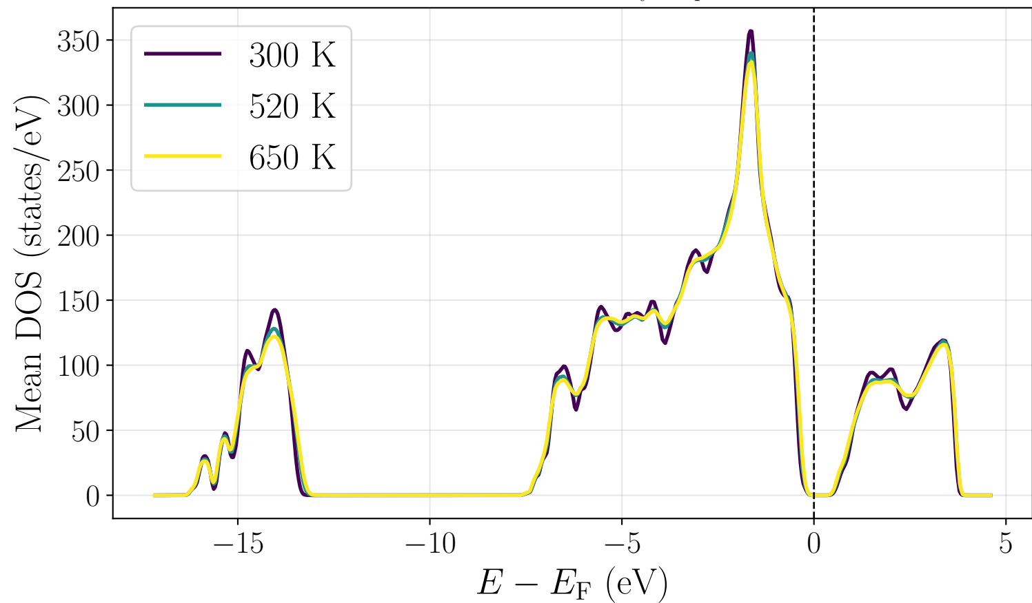
Ensemble-mean total DOS by temperature
