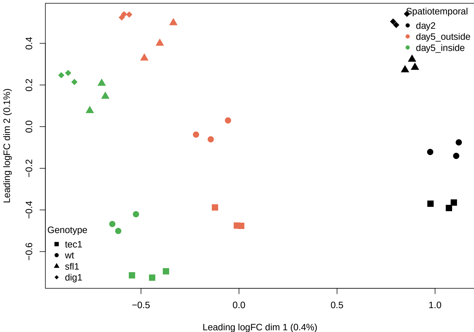
MDS plot of RNA-seq samples
