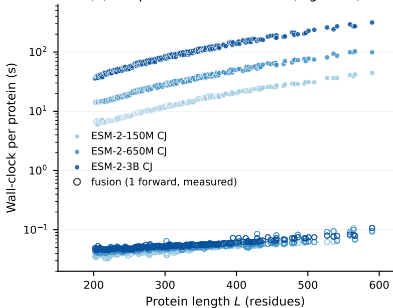
(a) Per-protein wall-clock vs L (log scale)
