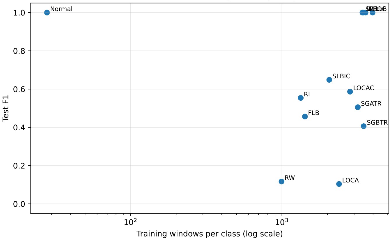
Per-class F1 vs. training-set frequency
