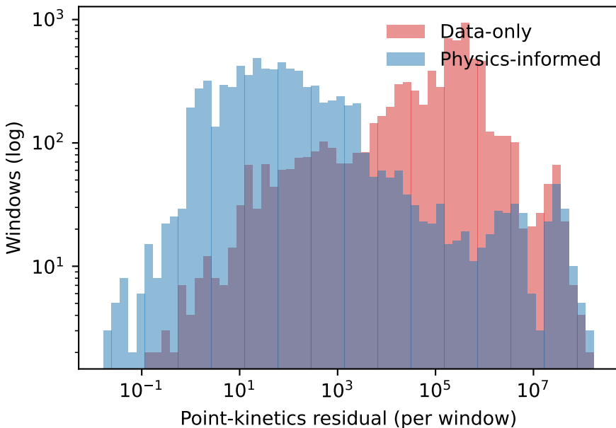
Point-kinetics residual
