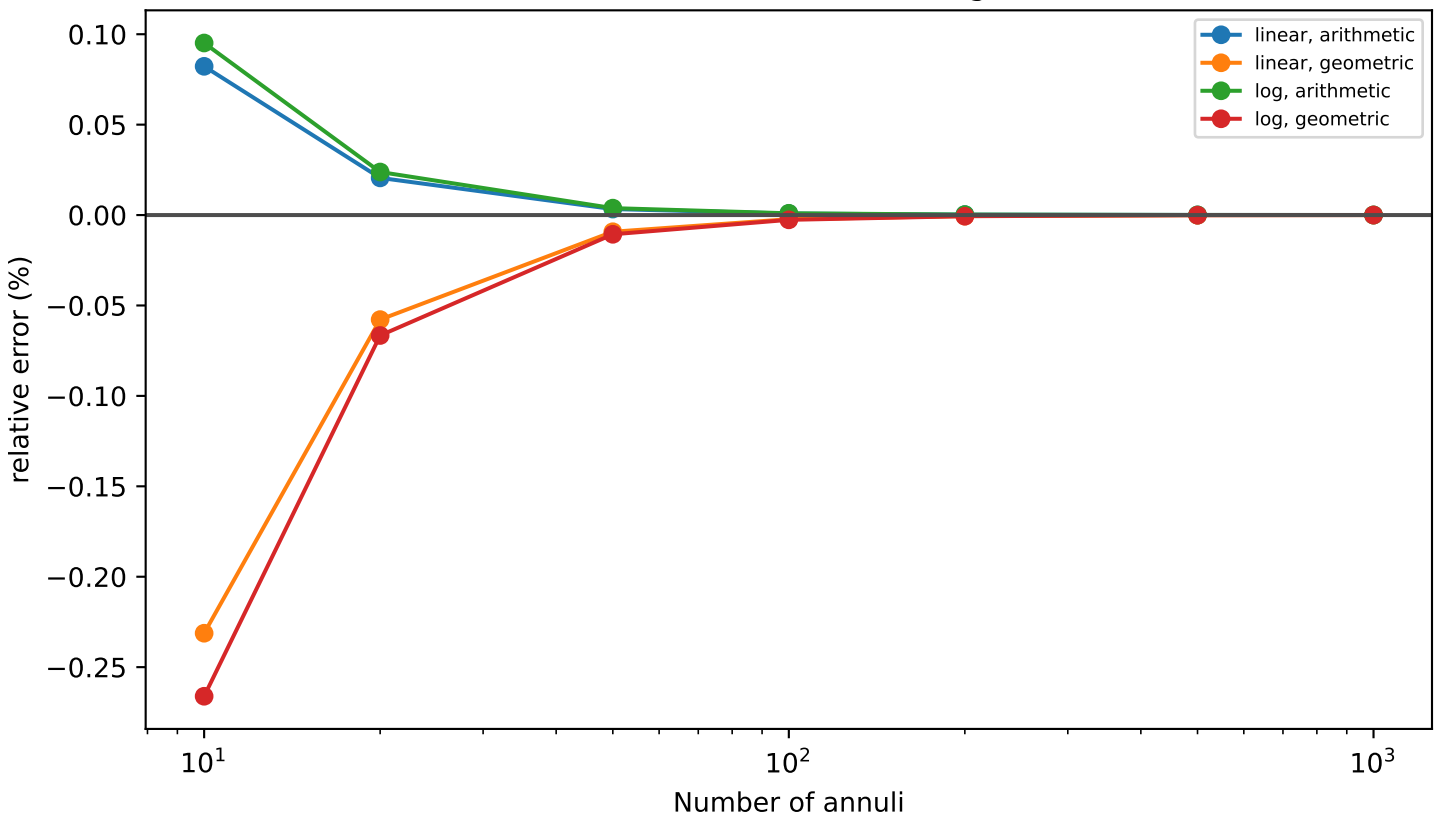
Broad-belt numerical convergence
