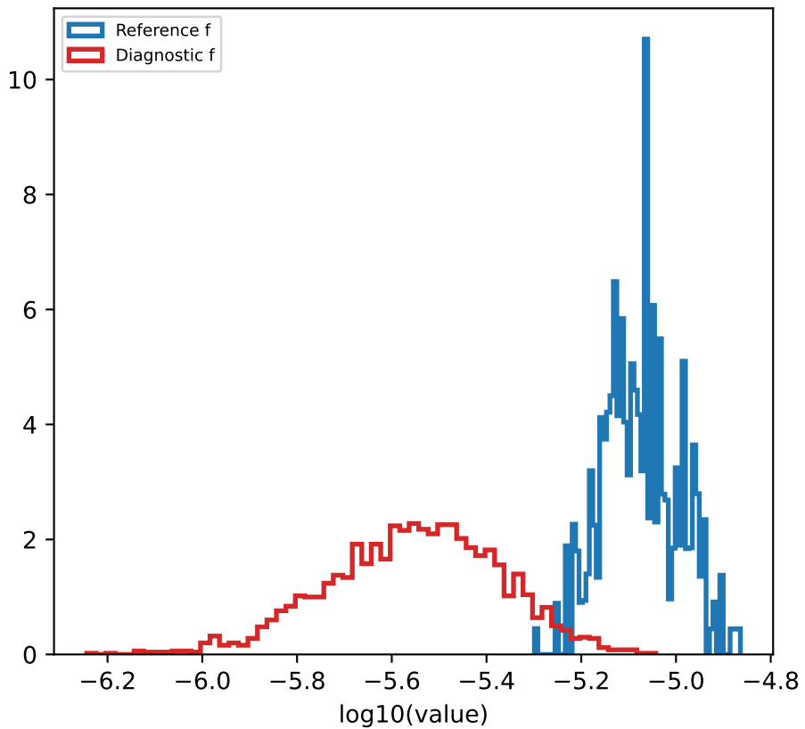
Fractional luminosity
