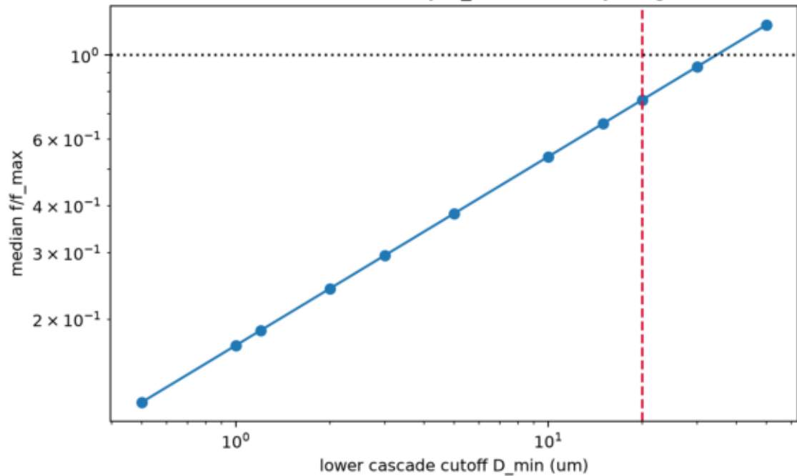
Reference luminosity D_min sensitivity (ring)
