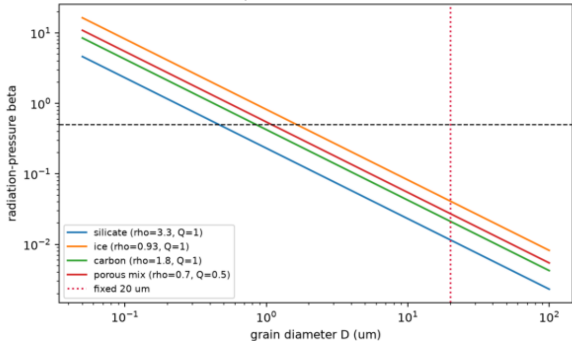
Radiation-pressure beta versus diameter
