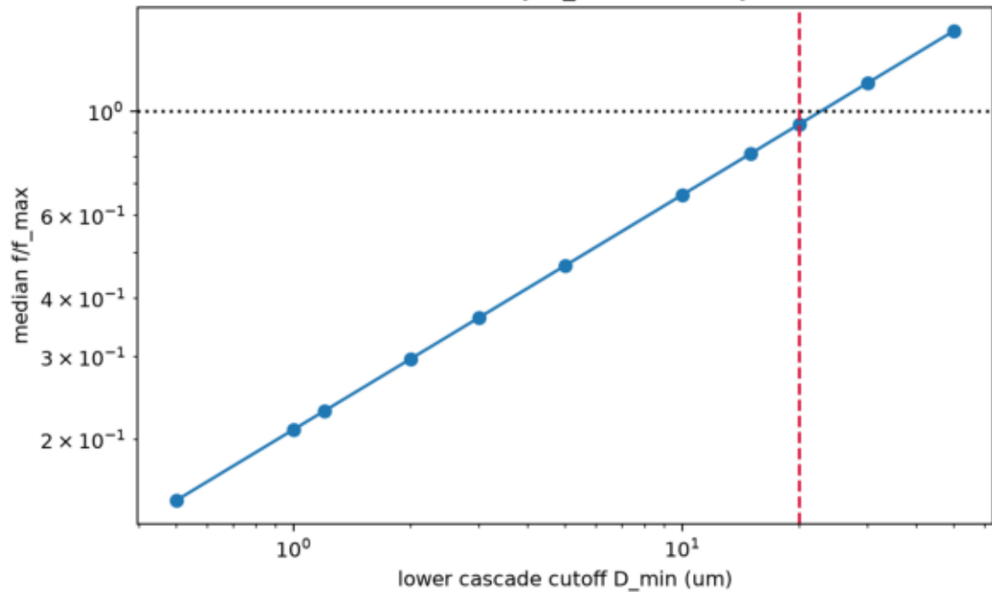
Reference luminosity D_min sensitivity (broad)
