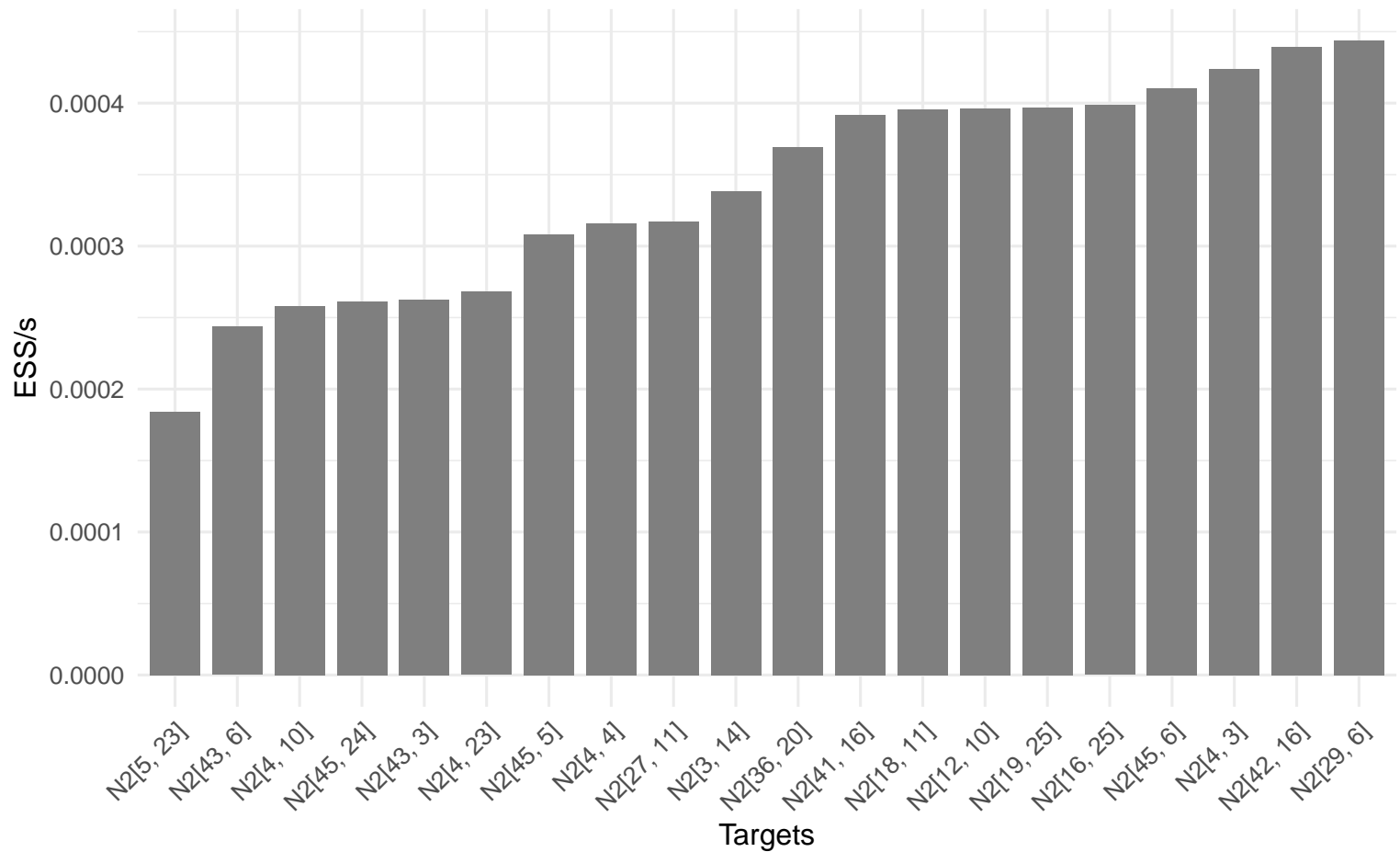
Worst Targets by Computational Efficiency (ESS/s)
