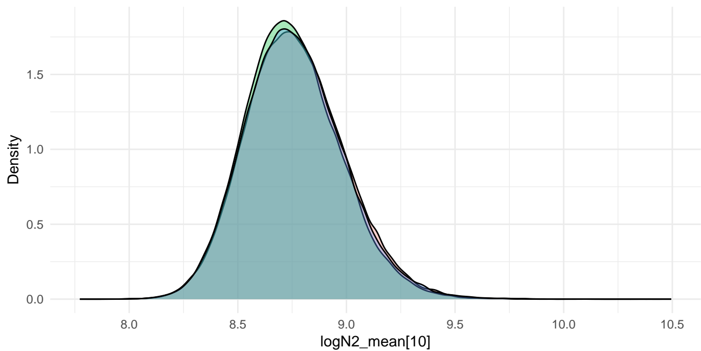
Density -- logN2_mean[10]
