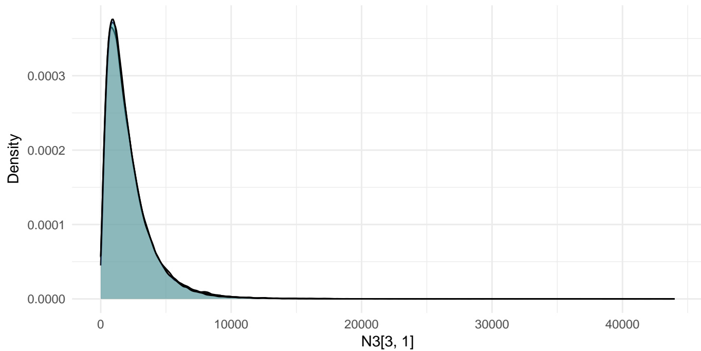
Density --- N3[3, 1]
