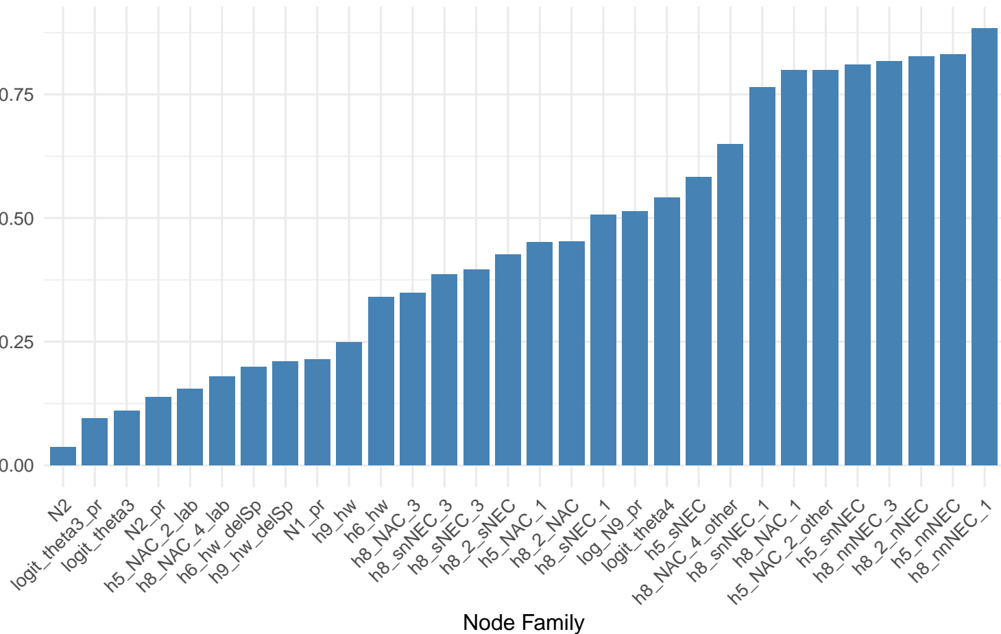
Median Algorithmic Efficiency by Node Family
