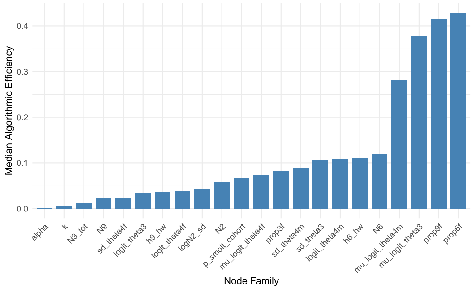
Median Algorithmic Efficiency by Node Family
