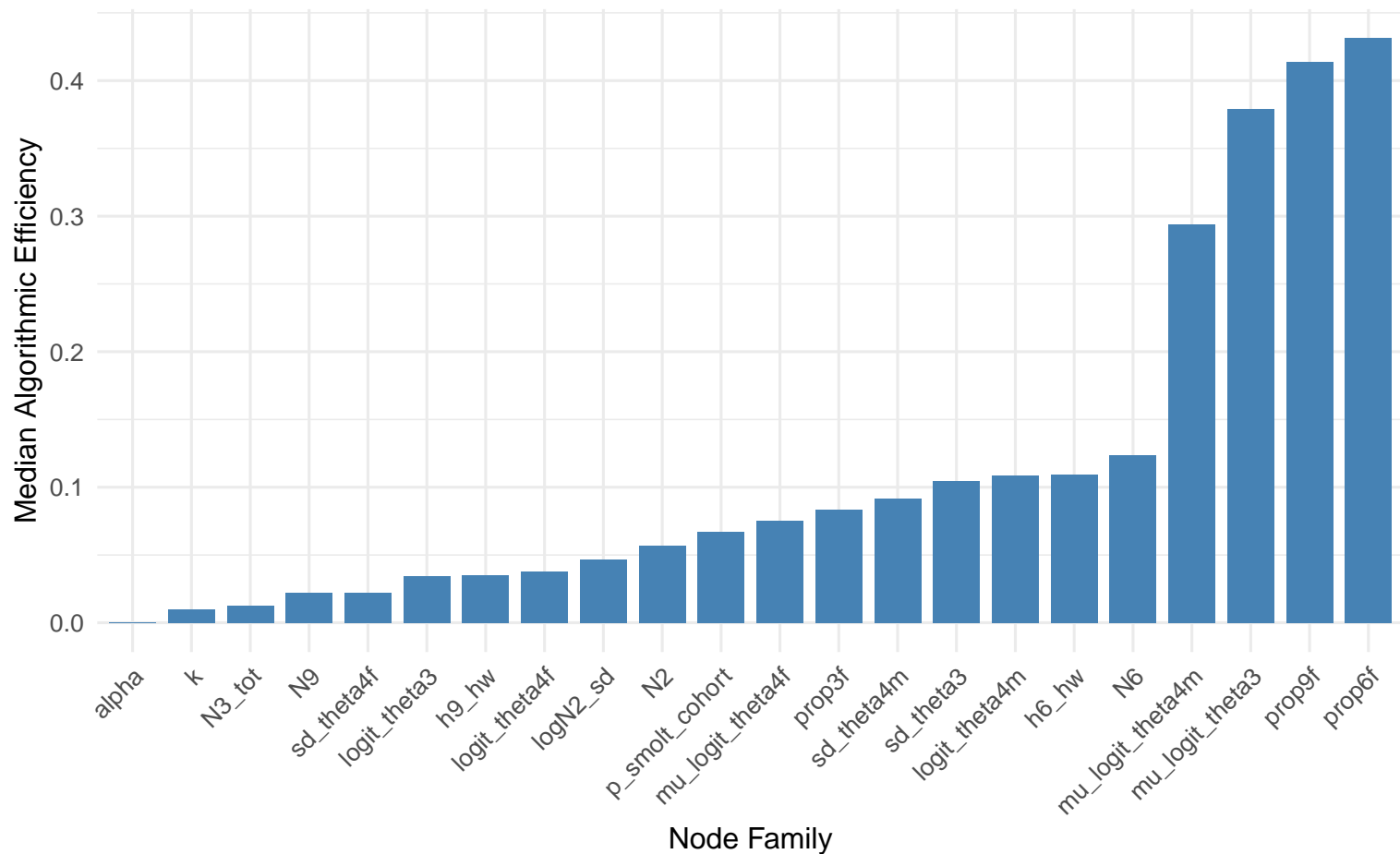
Median Algorithmic Efficiency by Node Family
