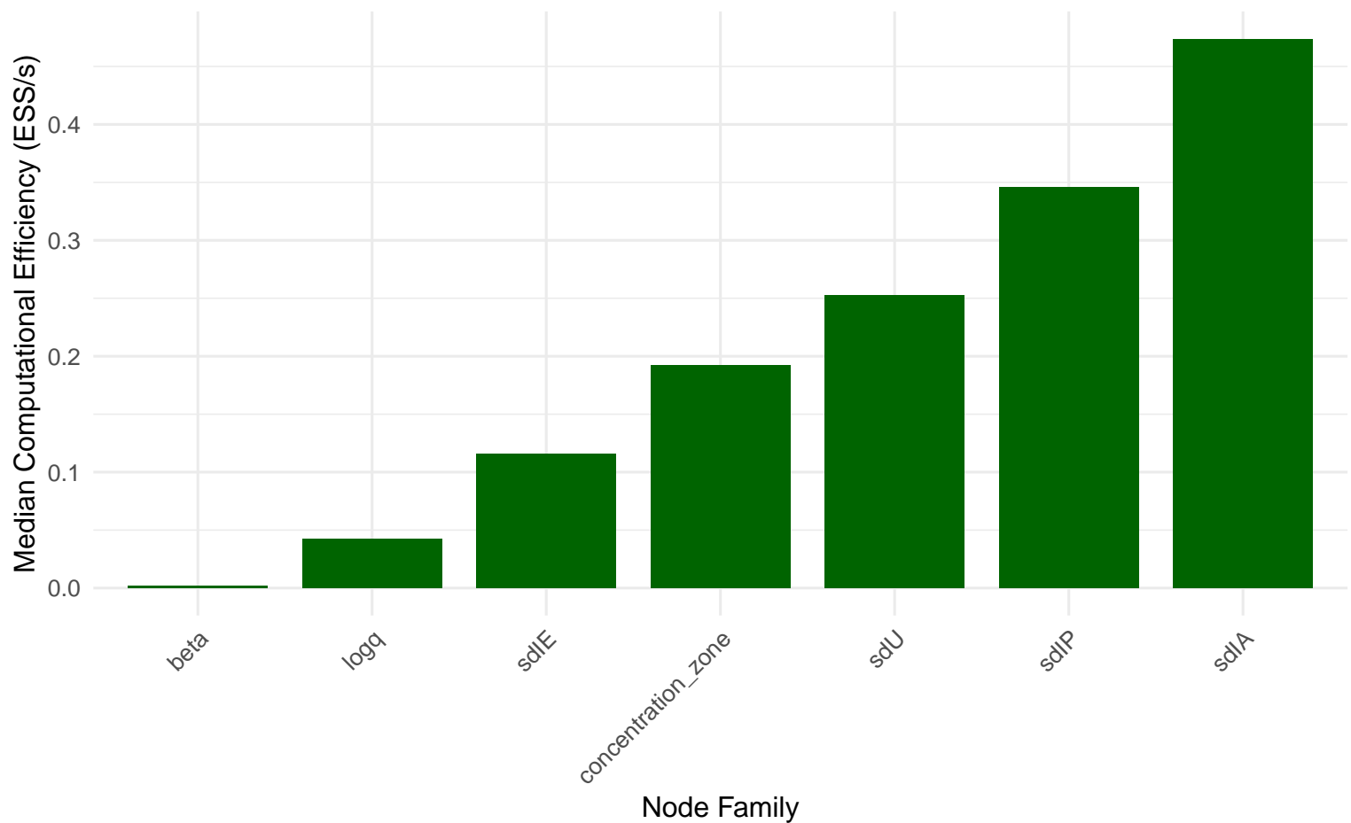
Median Computational Efficiency by Node Family
