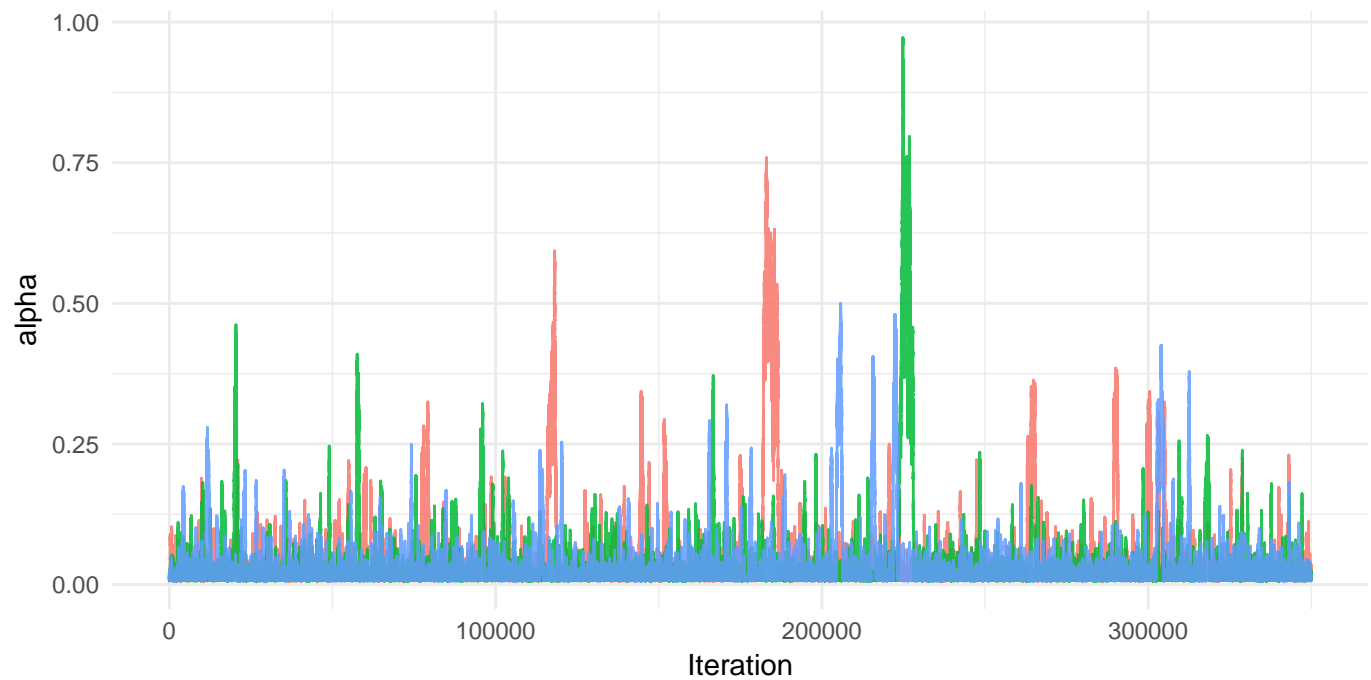
Density -- alpha
