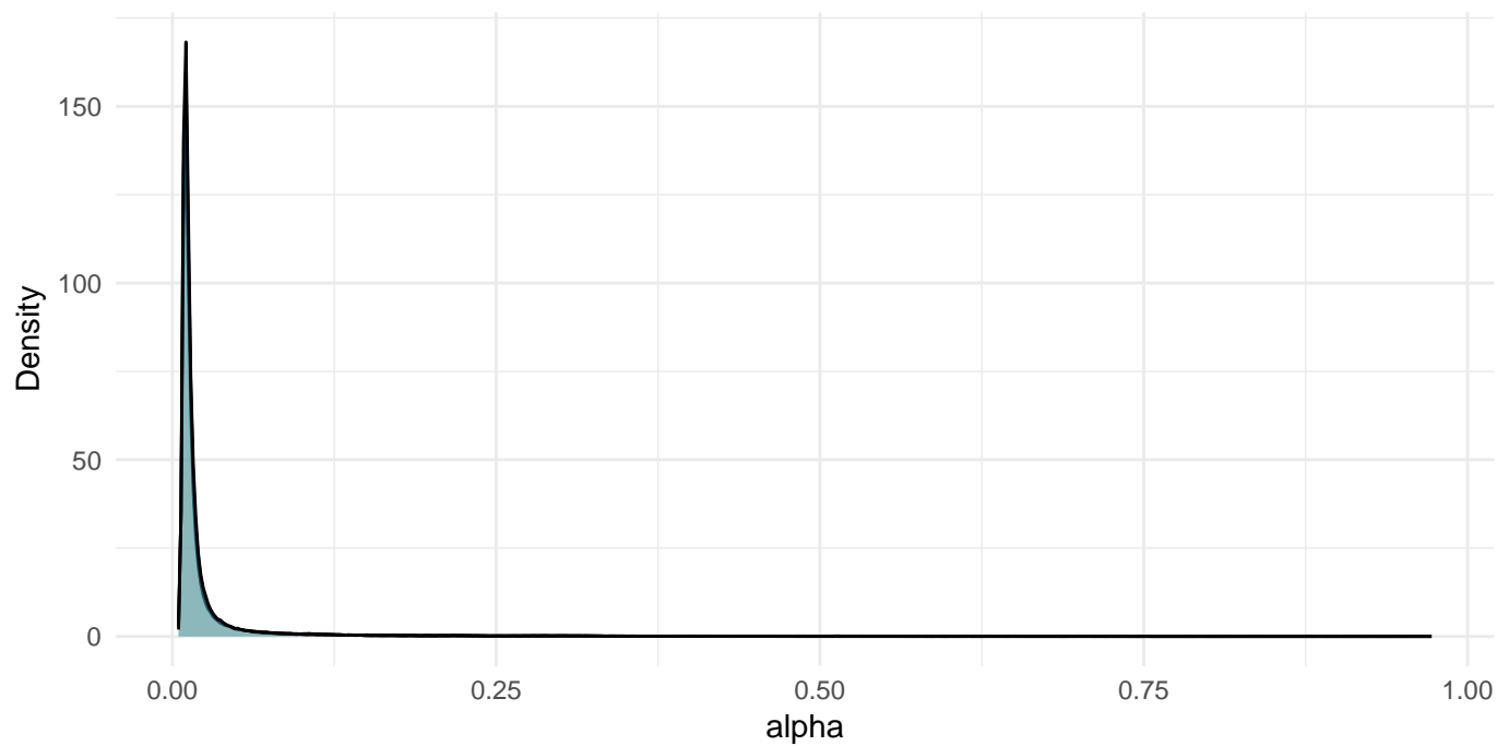
Density -- alpha
