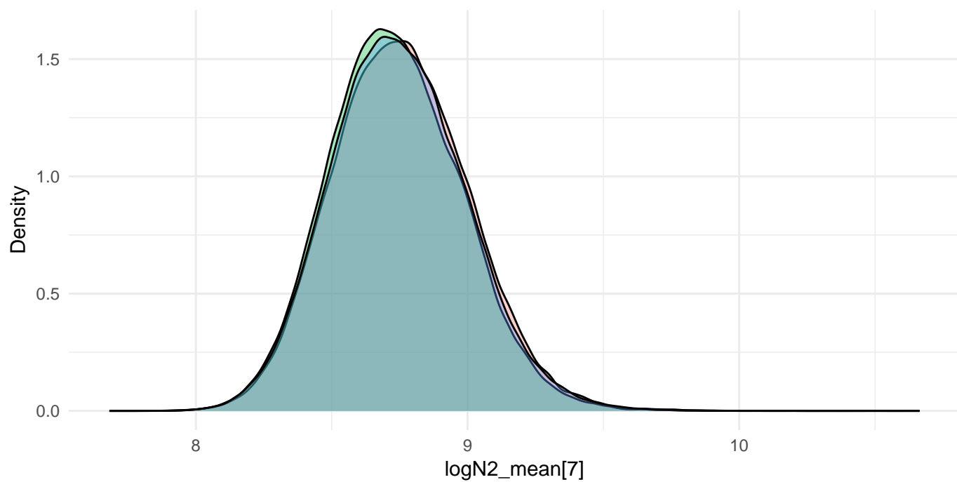
Density -- logN2_mean[7]
