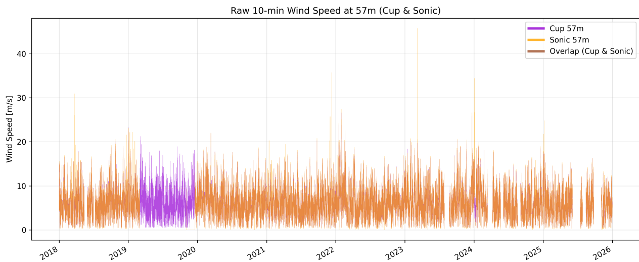
Figure 3: Raw 10-minute wind speed at 57m from the Cup and Sonic anemometers.
