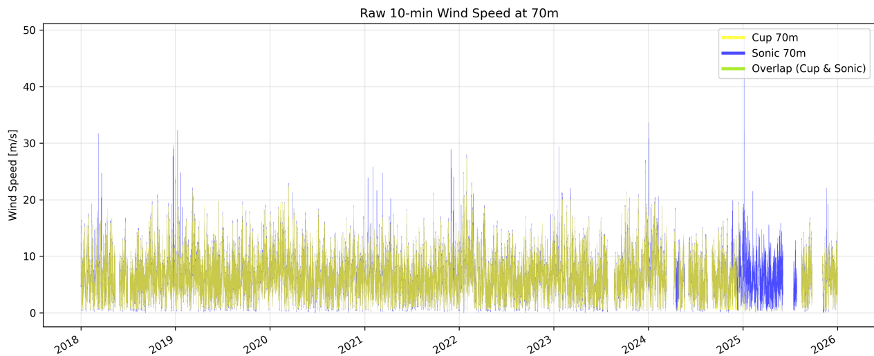
Figure 2: Raw 10-minute wind speed at 70m from the Cup and Sonic anemometers.
