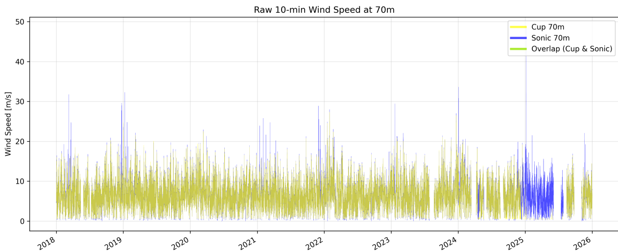
Figure 3: Raw 10-minute wind speed at 70m from the Cup and Sonic anemometers.
