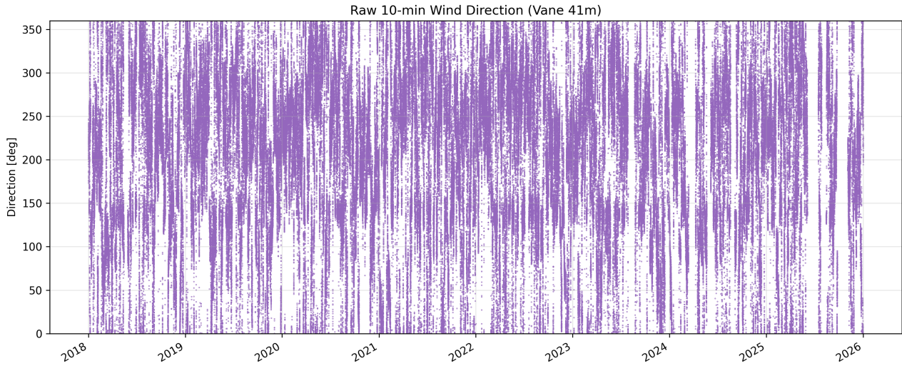
Figure 7: Wind direction time series from the wind vane at 41m height.
