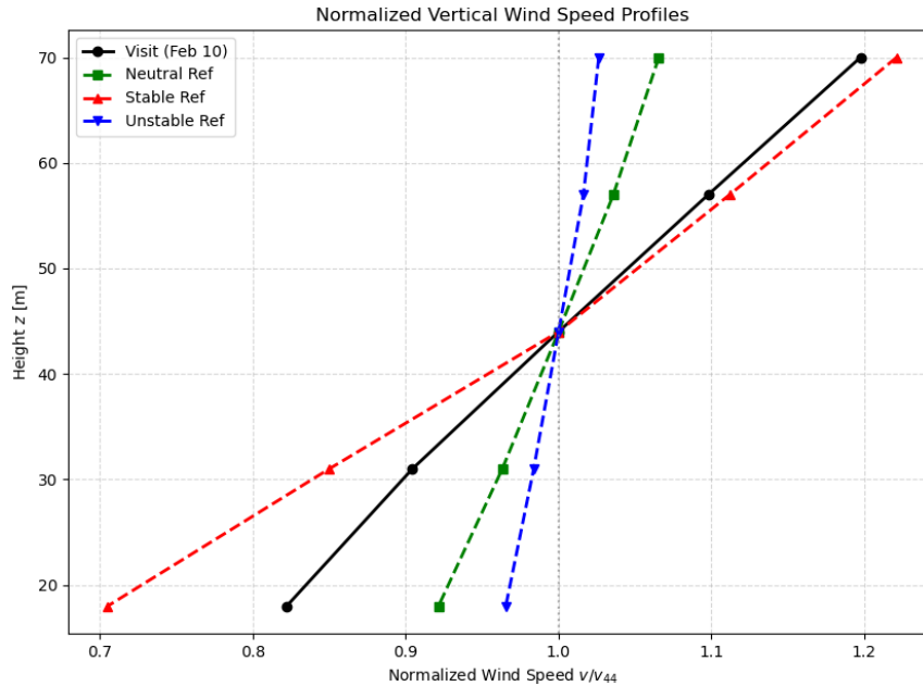
Figure 1: Normalized wind speed profiles v/v_{44} for the visit day compared to DTU reference datasets.
