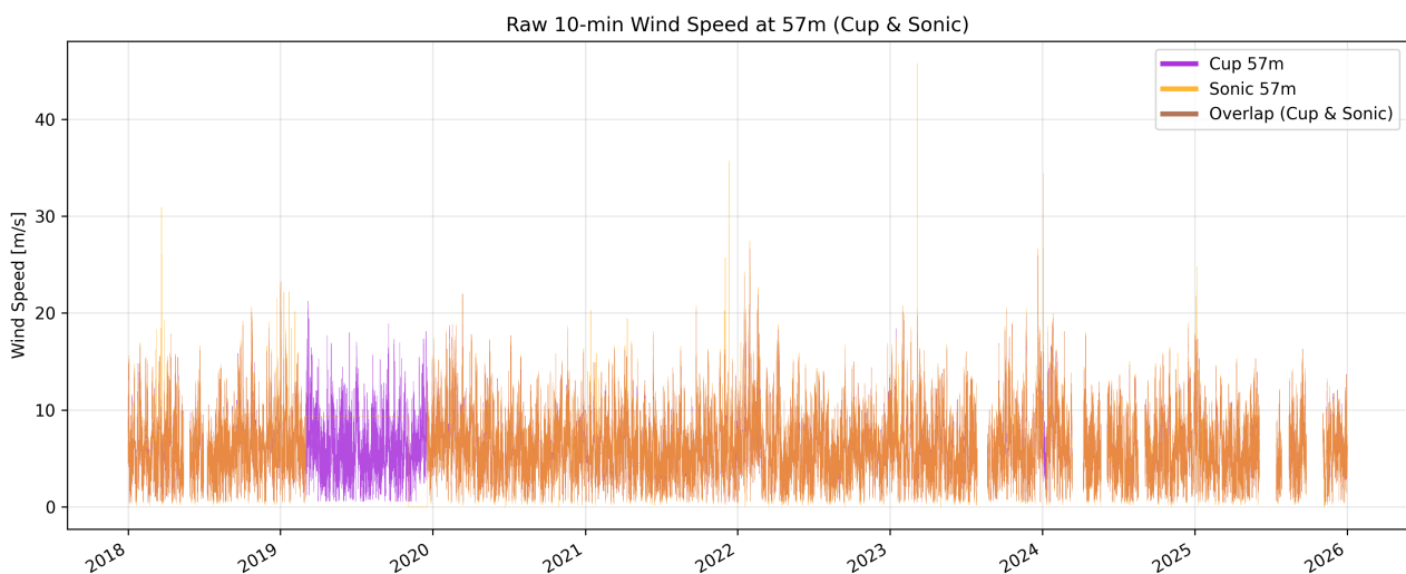
Figure 4: Raw 10-minute wind speed at 57m from the Cup and Sonic anemometers.
