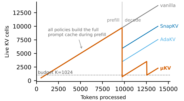
Figure 2: Live KV cells through prefill and decode on Llama-3.2-1B, phone CPU. Every policy builds the full prompt cache. Neither per-head evictor returns to its budget; \mu KV compacts to 721 cells and its re-eviction holds the cache near 2K.
