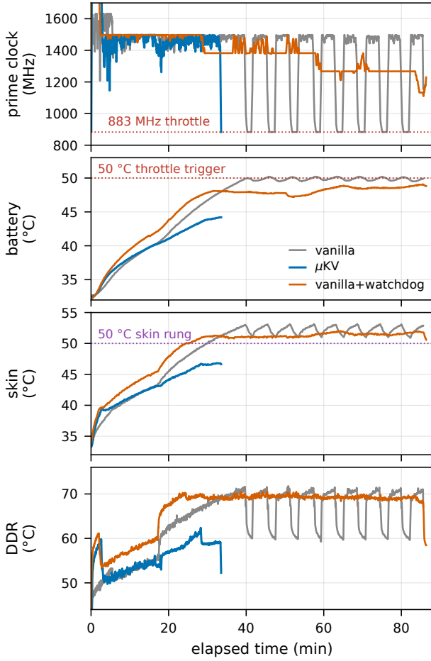
Figure 5: Bonsai-8B on the CPU from a cold start: prime clock, battery, skin and DDR for the full cache, \mu KV, and the full cache with the watchdog (ablation).
