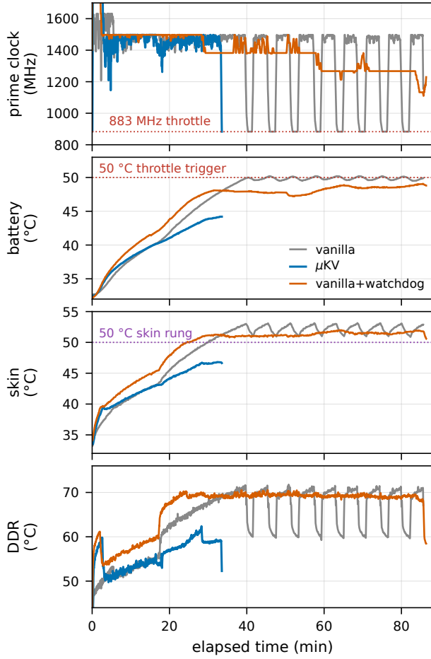
Figure 4: Bonsai-8B on the CPU from a cold start: prime clock, battery, skin and DDR for the full cache, \mu KV, and the full cache with the watchdog (ablation).
