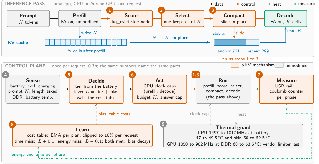
Figure 1: \mu KV on the phone. Top: the inference pass; scoring, selection and compaction (1 to 3) are the only changes. Bottom: the control plane, once per request. The same nine numbers name the same parts.
