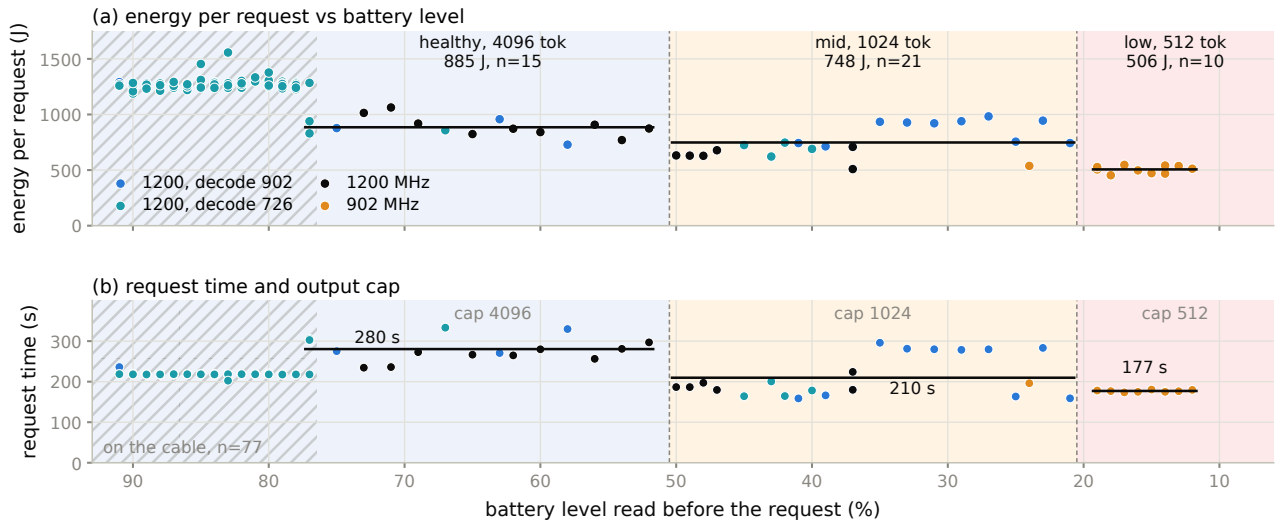
Figure 6: The scheduler through a real discharge: energy and time per request against the battery level it read, with tier bands, the plan chosen and the answer cap. Hatched: cable in.
