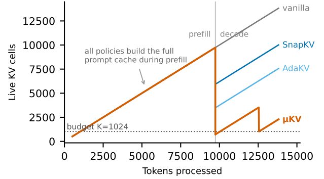
Figure 3: Live KV cells through prefill and decode, Llama-3.2-1B on the phone CPU. Every policy builds the full prompt cache. Neither per-head evictor returns to its budget; \mu KV compacts to 721 and holds near 2K.
